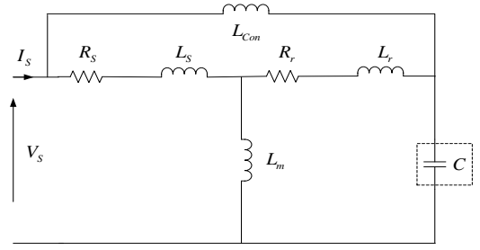
Fig. 5 High frequency model of DFIG
