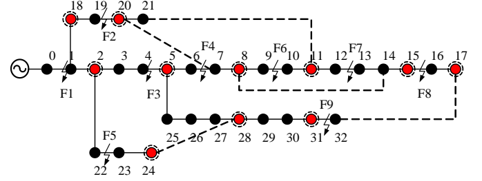
Fig.8 Configuration of the tested distribution system with DFIGs
