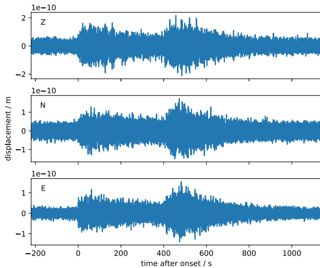
Figure 3. Three component displacement seismogram for S0421a filtered in the frequency range 0.5–7 Hz. The telltale sign of an HF event are the two distinct energy pulses that are separated by up to several minutes, both of which have an emergent onset and a long coda. HF, high frequency.
