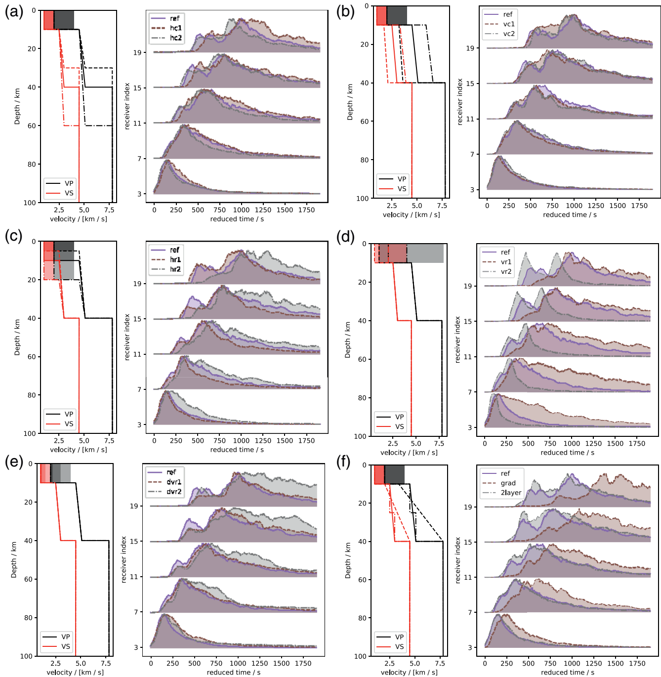
Figure 14. Sensitivity analysis for synthetic envelopes to changes in (a) crustal thickness and (b) velocities, (c) shallow layer thickness, (d) velocities and (e) scattering strength. (f) shows a model without a first order discontinuity at the moho and one with two crustal layers. Receivers are placed such that the estimated guided phase traveltimes based on the fastest crustal velocities are similar and hence the envelopes more directly comparable in time.
