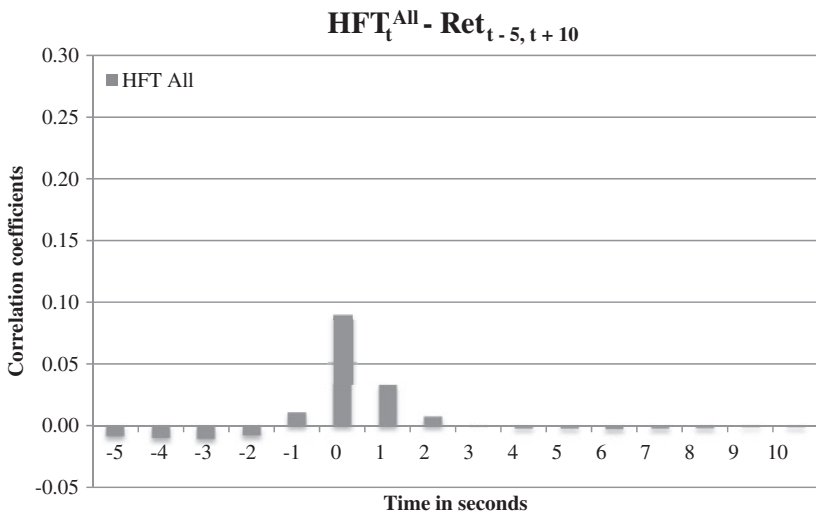
Figure 1 Overall correlation of HFT and returns
