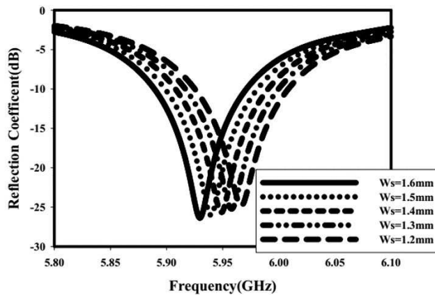
Figure 9. Reflection characteristics versus W_s ( L=40\text{mm} , a=16\text{mm} , W=8.613\text{mm} , H=0.254\text{mm} )
