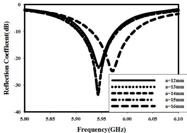
Figure 10. Reflection characteristics versus a ( L=40\text{mm} , H=0.254\text{mm} , W=8.613\text{mm} , W_s=1.2\text{mm} )
