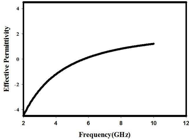
Figure 2. Effective permittivity curve
