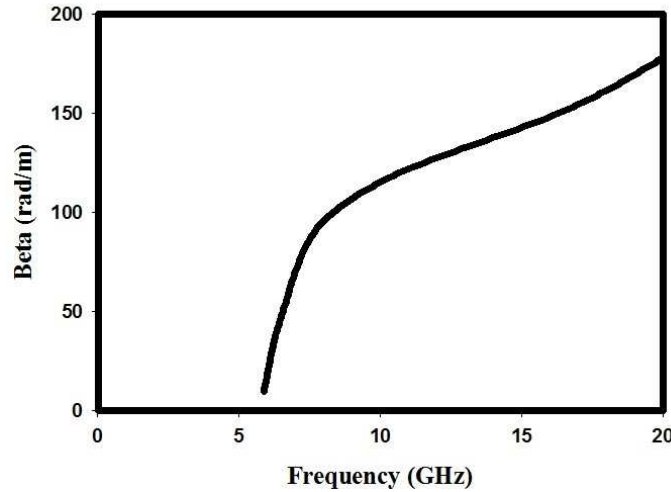
Figure 4. Dispersion diagram
