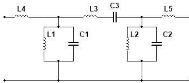
Figure 5. Equivalent circuit model
