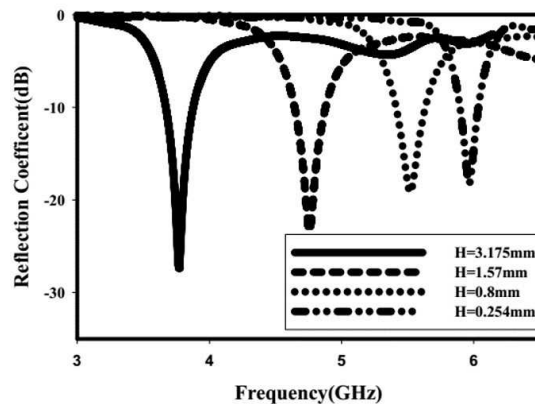
Figure 6. Reflection characteristics versus substrate height ( L=40 mm, a=16 mm, W=8.613 mm, W_s=1.2 mm)
