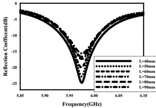
Figure 11. Reflection characteristics versus L ( H=0.254\text{mm} , a=16\text{mm} , W=8.613\text{mm} , W_s=1.2\text{mm} )
