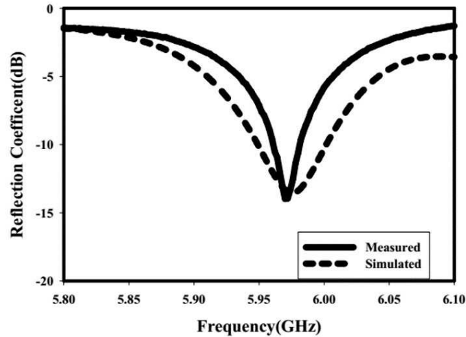
Figure 14. Reflection Characteristics
