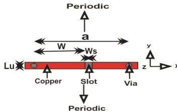
Figure 3. Unit cell
