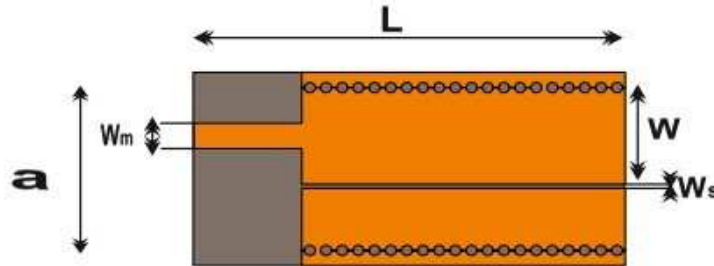
Figure 1. Single SIW ENZ antenna
