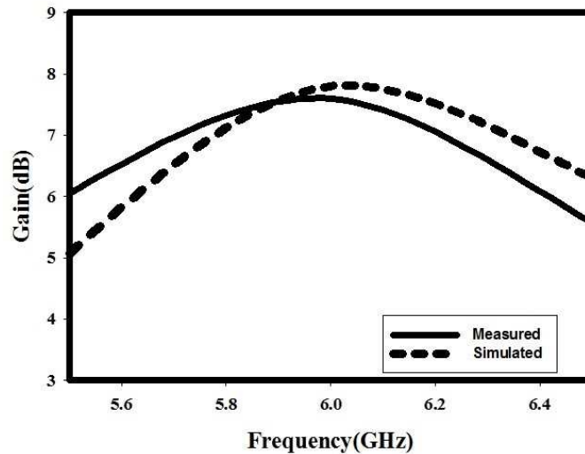
Figure 15. Measured and Simulated Gain
