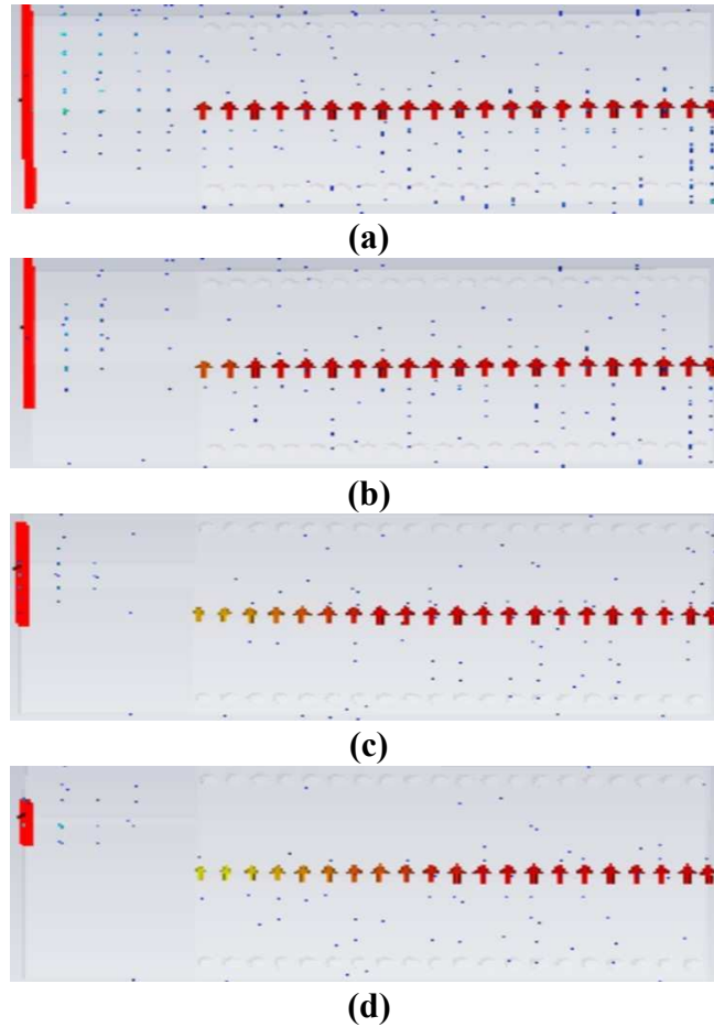
Figure 7. E-field distribution (a) H=3.175 mm (b) H=1.575 mm (c) H=0.8 mm (d) H=0.254 mm ( L=40 mm, a=16 mm, W=8.613 mm, W_s=1.2 mm)
