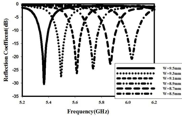
Figure 8. Reflection characteristics versus W ( L=40\text{mm} , a=16\text{mm} , H=0.254\text{mm} , W_s=1.2\text{mm} )
