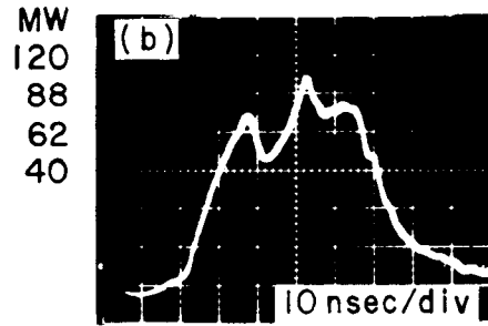
rf Into Accelerator
