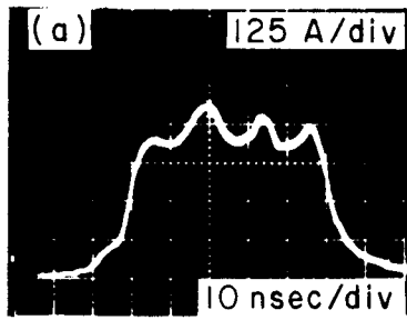
1- MeV Klystron Beam
