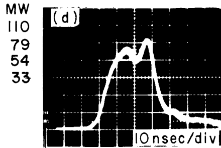
rf Out of Accelerator
