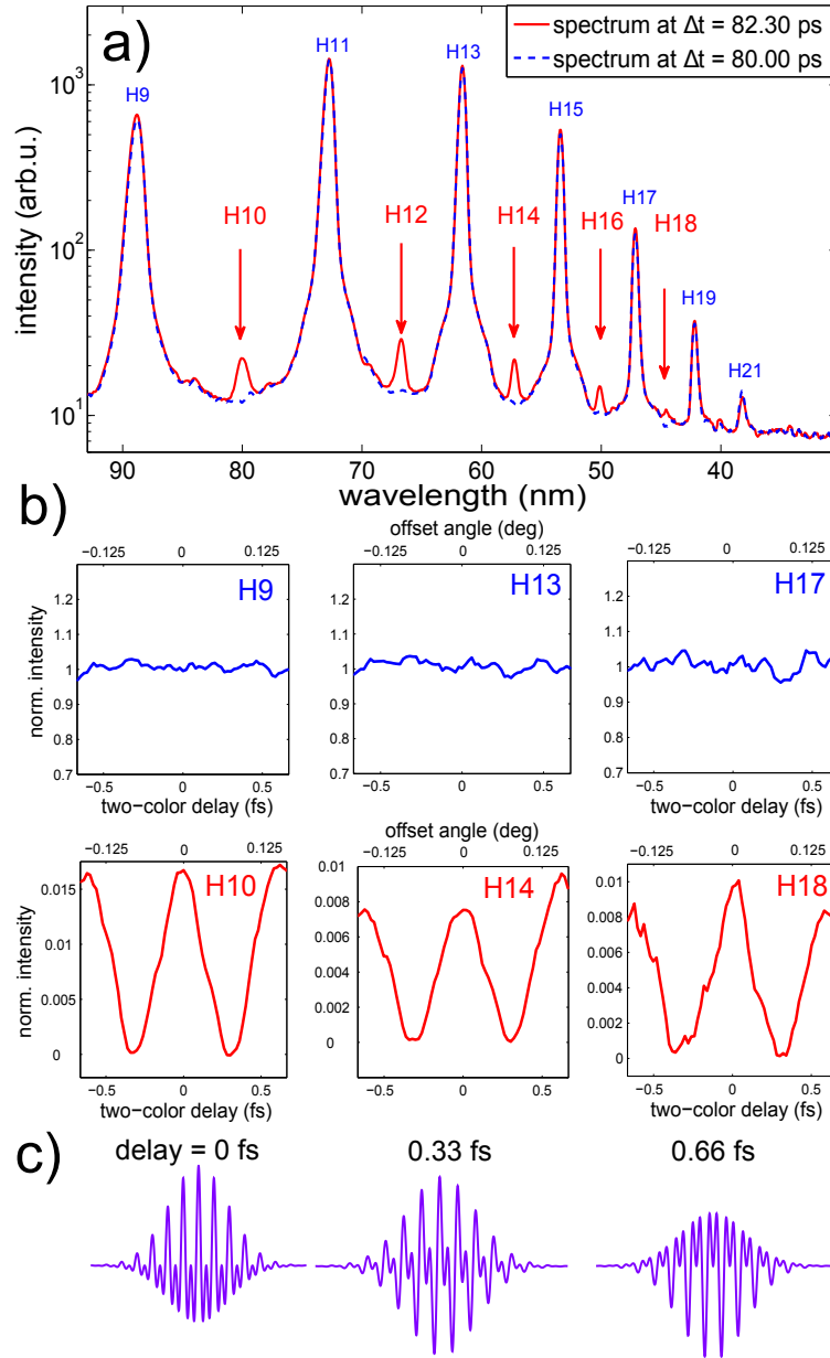
FIG. 2: a) High-harmonic spectra recorded at pump-probe delays of 82.3 ps (maximal orientation, red line), showing the presence of the even harmonics H10-H18 emitted from oriented molecules and 80.0 ps (near-random distribution of molecules, blue dashed line). b) Variation of the intensity of the odd harmonics (blue lines) and even harmonics (red lines) as a function of the sub-cycle temporal delay between the 800 nm and 400 nm laser fields forming the pump pulse. The corresponding offset angle of the 0.7 mm calcite plate is given on the top axis. The intensity of the odd harmonics has been normalized to their value at \Delta t = 80.0 ps and the intensity of each even harmonic H_{2n} has been divided by the intensity at \Delta t=80.0 ps of the next lower odd harmonic H_{2n-1} . c) Schematic illustration of the electric field of a 800+400 nm laser pulse for different two-color delays.
