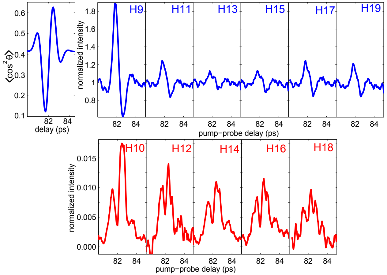
FIG. 3: Variation of the intensity of the odd harmonics (H9-H19, blue lines) and even harmonics (H10-H18, red lines) with pump-probe delay. The intensity of the odd harmonics has been normalized to their value at \Delta t=80.0 ps and the intensity of each even harmonic H_{2n} has been divided by the intensity, at \Delta t=80.0 ps, of the next lower odd harmonic H_{2n-1} . The calculated evolution of the degree of axis alignment is shown in the upper left panel.
