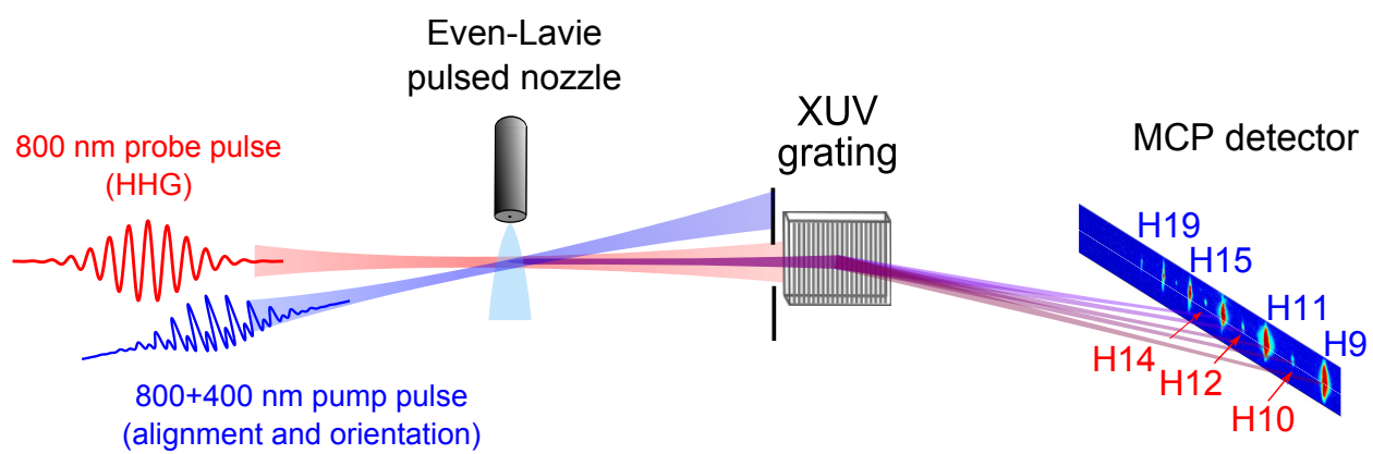
FIG. 1: Experimental setup for high-harmonic spectroscopy of oriented molecules. The illustration of the laser pulses is schematic. The far-field spectrally resolved high-harmonic profile is a false-color logarithmic plot obtained at maximal orientation of the OCS molecules.
