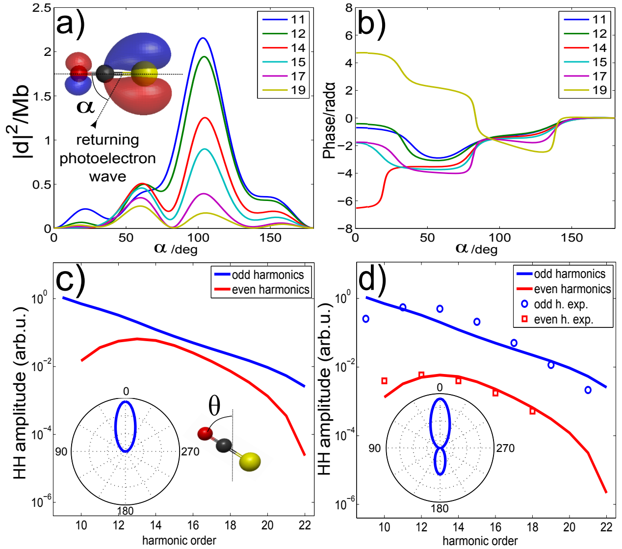
FIG. 4: a) and b) Calculated photorecombination matrix elements for the HOMO of OCS using ab initio quantum scattering theory. The inset shows the HOMO of OCS as an isocontour plot and color-coded sign. c) Predicted high-harmonic spectra for the odd orders (blue line) and even orders (red line) using the matrix elements from a) and b) and the axis distribution shown as inset ( \langle \cos^2 \theta \rangle = 0.63 , perfect head-to-tail order). d) Measured and calculated intensities of the odd and even harmonic orders using the axis distribution shown in the inset ( \langle \cos^2 \theta \rangle = 0.63 , 30% head-to-tail order), obtained by fitting the head-to-tail order in the calculation to the experimental data.
