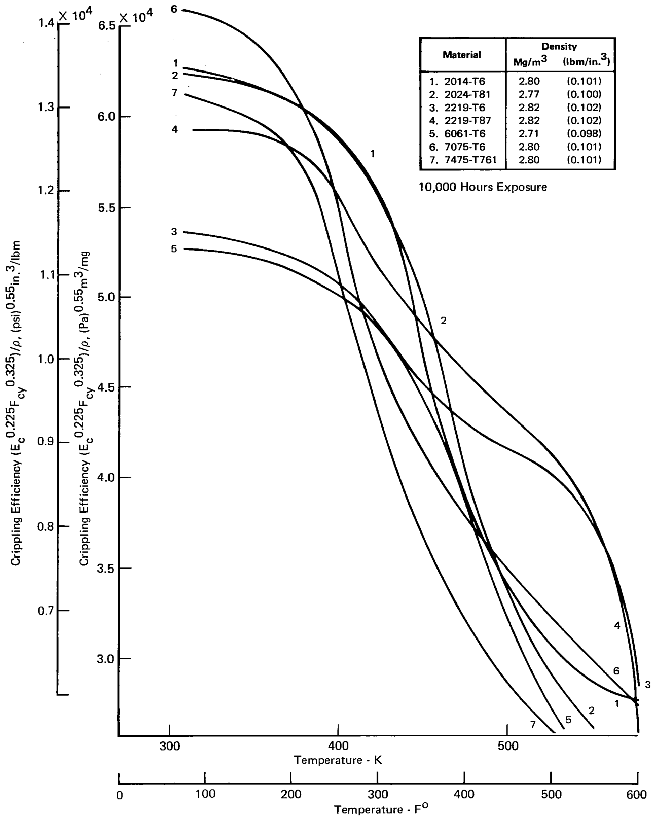
FIGURE 24 ALUMINUM CRIPPLING EFFICIENCY vs TEMPERATURE
