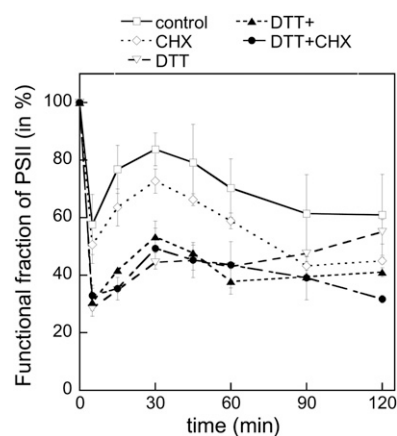
Figure 4. Functional fraction of PSII (in percentage) during 2 h of HL treatment as an indicator of PSII photoinactivation calculated by 1/F_0 - 1/F_m . The ratio 1/F_0 - 1/F_m obtained before the start of the light treatment was taken as 100%. For definitions, see Figure 3. DTT+CHX, DTT (500 \mu\text{M} ) and CHX (2 \mu\text{g mL}^{-1} ) were added 15 and 45 min before light exposure, respectively.
