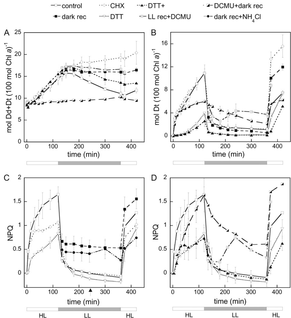
Figure 3. Dd+Dt (A) and Dt (B) content and NPQ (C and D) during 2 h of HL treatment, 4 h of LL recovery, and subsequently 1 h of HL treatment. Control, Cultures without inhibitors; dark rec, after 2 h of HL exposure, 4 h of darkness followed instead of 4 h of LL; CHX, cultures were incubated with 2 \mu\text{g mL}^{-1} CHX for 45 min before starting the experiment; DTT, cultures were incubated with DTT (500 \mu\text{M} ) for 15 min before starting the experiment; DTT+, DTT (500 \mu\text{M} ) was added additionally every 20 min during the HL treatment and 20 min before the second HL treatment; LL rec+DCMU, DCMU (10 \mu\text{M} ) was added before starting the LL recovery period; DCMU+dark rec, DCMU (10 \mu\text{M} ) was added 10 min before light exposure, and recovery was performed in darkness; dark rec+ \text{NH}_4\text{Cl} , recovery was performed in darkness, and after 2 h of darkness, \text{NH}_4\text{Cl} (5 mM) was added (indicated with the arrow). Samples represent means of two to five independent experiments \pm SD, except for the NPQ values of DCMU-treated samples during the recovery time, where only one experiment was performed.
