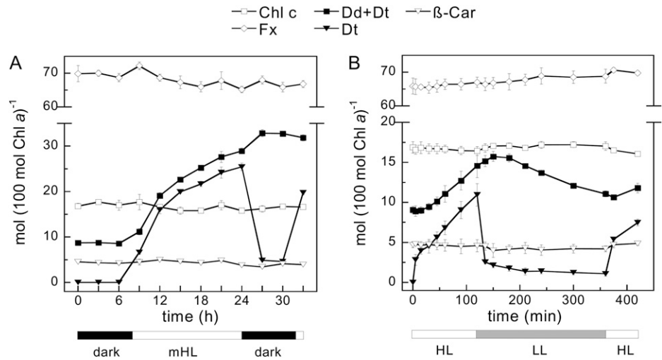
Figure 2. Pigment evolution during the mHL (A) and HL (B) experiments. In A, the recovery period was performed at darkness, while in B, recovery was monitored at LL conditions. After 4 h of recovery from HL, cells were again exposed to 1 h of HL treatment. Values are means of three (A) and five (B) independent experiments \pm SD. \beta -Car, \beta -Carotene.
