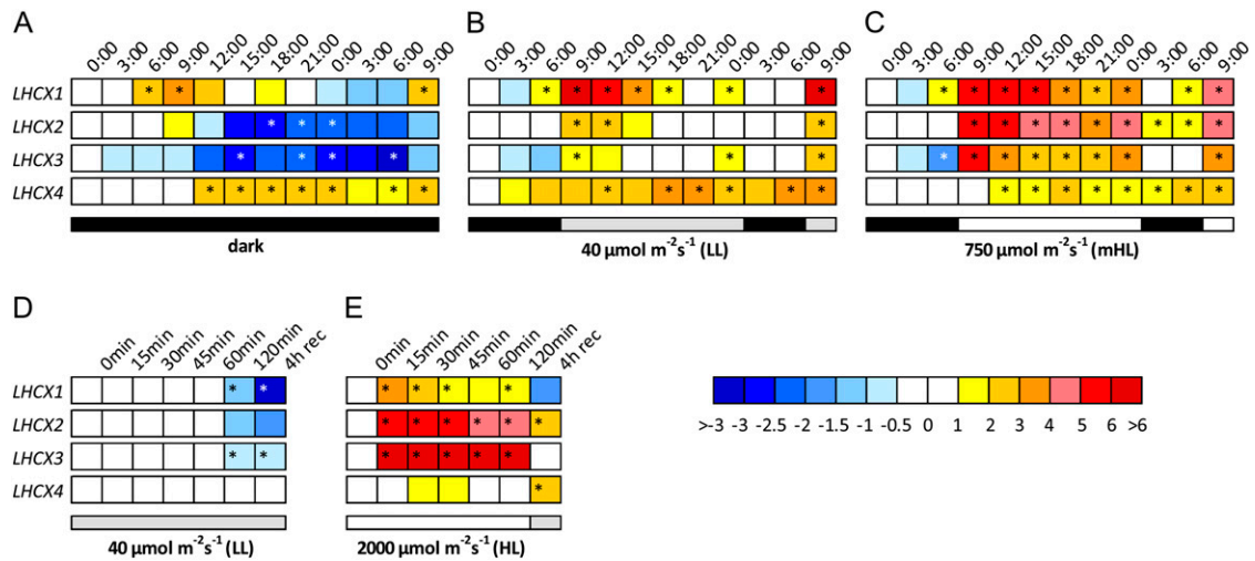
Figure 1. LHCX transcription levels in different light regimes. Expression ratios are given in \log_2 -transformed values as indicated by the color bar and represent relative amounts with reference to 18S gene expression. All levels were normalized to the respective initial value and represent means of four independent measurements. Asterisks represent significant changes at P < 0.05 (Pairwise Fixed Reallocation Randomization Test performed by REST). A to C, A 33-h experiment with darkness all the time (A), 40 \mu\text{mol photons m}^{-2} \text{s}^{-1} illumination (LL) from 8 AM until 12 AM (B), and 750 \mu\text{mol photons m}^{-2} \text{s}^{-1} illumination (mHL) from 8 AM until 12 AM (C). D and E, A 6-h experiment with LL illumination all the time (D) and 2,000 \mu\text{mol photons m}^{-2} \text{s}^{-1} illumination (HL) for the first 2 h followed by 4 h of LL recovery (E).
