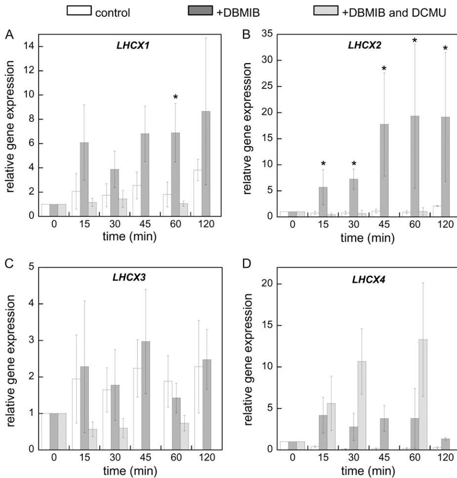
Figure 7. Relative gene expression of LHCX1 (A), LHCX2 (B), LHCX3 (C), and LHCX4 (D) during illumination with LL_{100} . Relative LHCX transcription levels with reference to 18S gene expression were normalized to the initial amount. White bars, no chemical treatment; dark gray bars, 1 \mu\text{M} DBMIB was applied 10 min before the light treatment; light gray bars, in addition to DBMIB, 10 \mu\text{M} DCMU was applied 10 min before the light treatment. Analyses were performed at the indicated time points, and values represent means of three independent samples \pm SD. Asterisks represent significant differences ( P < 0.05 ; Pairwise Fixed Reallocation Randomization Test performed by REST) of the DBMIB-treated samples compared with the respective control samples and, when available, also compared with the respective DBMIB- + DCMU-treated samples. LHCX4 was significantly up-regulated in the presence of DBMIB compared with the control conditions at each time point. As this significance was abolished by comparing DBMIB-treated with DBMIB- + DCMU-treated samples, these are false-positive results; therefore, significance is also not indicated for time points 45 and 120 min.
