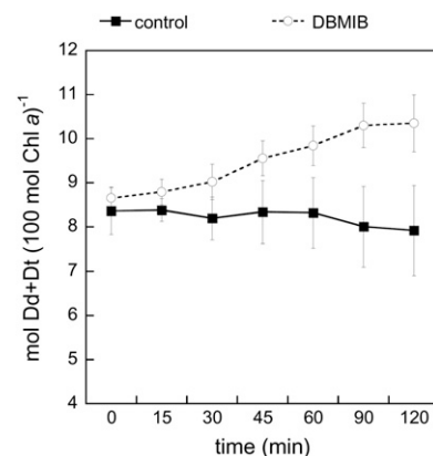
Figure 6. Evolution of the Dd+Dt pool size during illumination with \text{LL}_{100} . In these conditions, the Dt amount was less than 2% of the total Dd+Dt pool size in both experimental conditions. In the inhibitor treatment, 1 \mu\text{M} DBMIB was added 10 min before the start of the experiment. Depicted are mean values of four independent measurements \pm SD.
