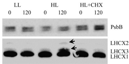
Figure 5. Western blot of LL-, HL-, and HL- + CHX-treated cultures. Indicated are the samples before (0) and after (120) 2 h of LL or HL treatment, respectively. A polyclonal LHCSR antibody of C. reinhardtii was employed, which detects all of the LHCX proteins. Arrows indicate LHCX2 and LHCX3, which can be distinguished from LHCX1 by their larger size. As a loading control, an antibody against the plastid-encoded PsbB (CP47) was applied.
