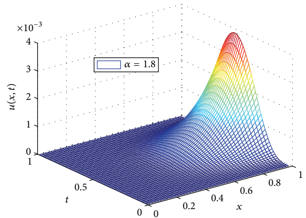
FIGURE 6: The analytical solution surface when \alpha = 1.8 in Example 3.
