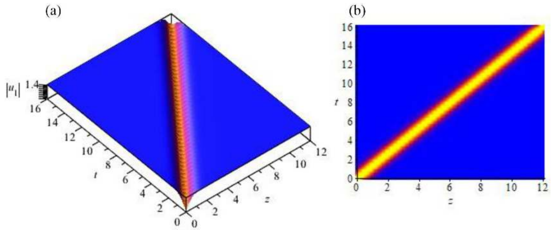
Fig. 1. The solution u_1(z, t) when b_0 = b_1 = \alpha_1 = \alpha_2 = \alpha_3 = 1 , \beta_1 = -2 , \beta_2 = 1 , and a = 2 : (a) 3D plot, (b) density plot.
