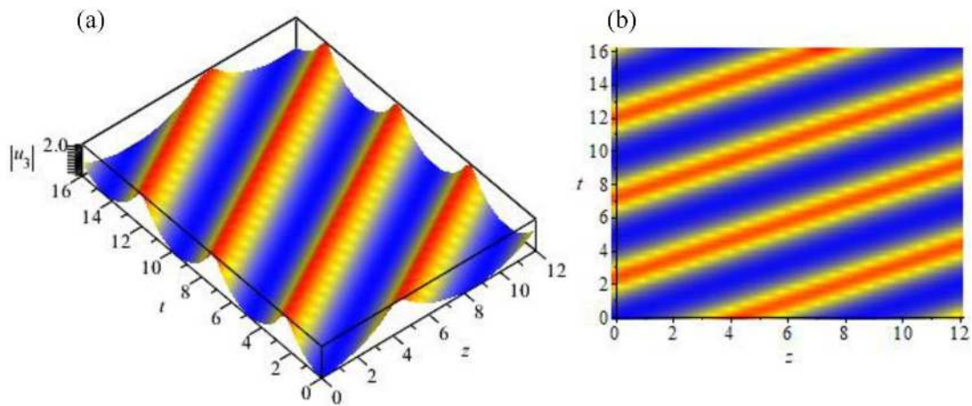
Fig. 2. The solution u_3(z, t) when b_0 = 1 , b_1 = 2 , \alpha_1 = 1.1 , \alpha_2 = 0.7 , \alpha_3 = 1.5 , \beta_1 = 1.9 , \beta_2 = 1 , and a = 2 : (a) 3D plot, (b) density plot.
