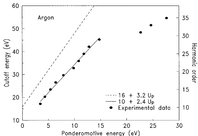
FIG. 11. Cutoff energy in argon as a function of the ponderomotive energy. The solid line is a linear best fit: 10 + 2.4U_p , the dashed line is the prediction of the single-atom response 16 + 3.2U_p .
