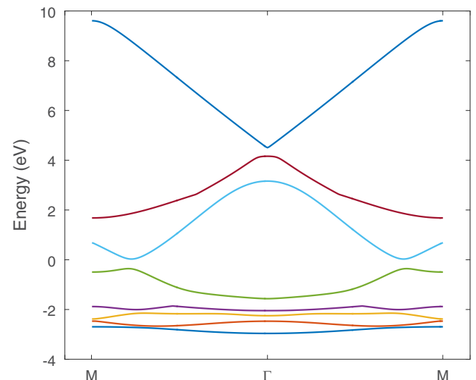
FIG. 6. ZnO band structure used in the simulations.
