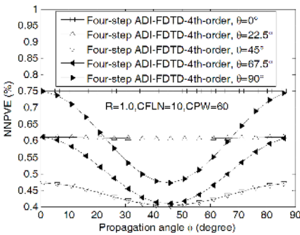
Figure 11. NNPVE versus \phi with CFLN = 10 and CPW = 60 for the proposed fourth-order scheme.
