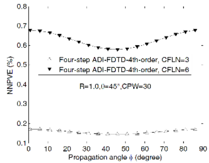
Figure 12. NNPVE versus \phi with \theta = 45^\circ and CPW = 30 for the proposed fourth-order scheme.
