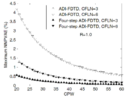
Figure 8. Maximum NNPVAE versus CPW with CFLN = 3, 6 for the second-order schemes.
