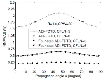
Figure 4. Normalized numerical phase velocity anisotropic error (NNPVAE) versus \phi with CFLN = 3, 6, CPW = 30 for the second-order schemes.
