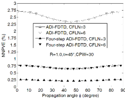
Figure 3. NNPVE versus \phi with CFLN = 3, 6, CPW = 30 and \theta = 45^\circ for the second-order schemes.
