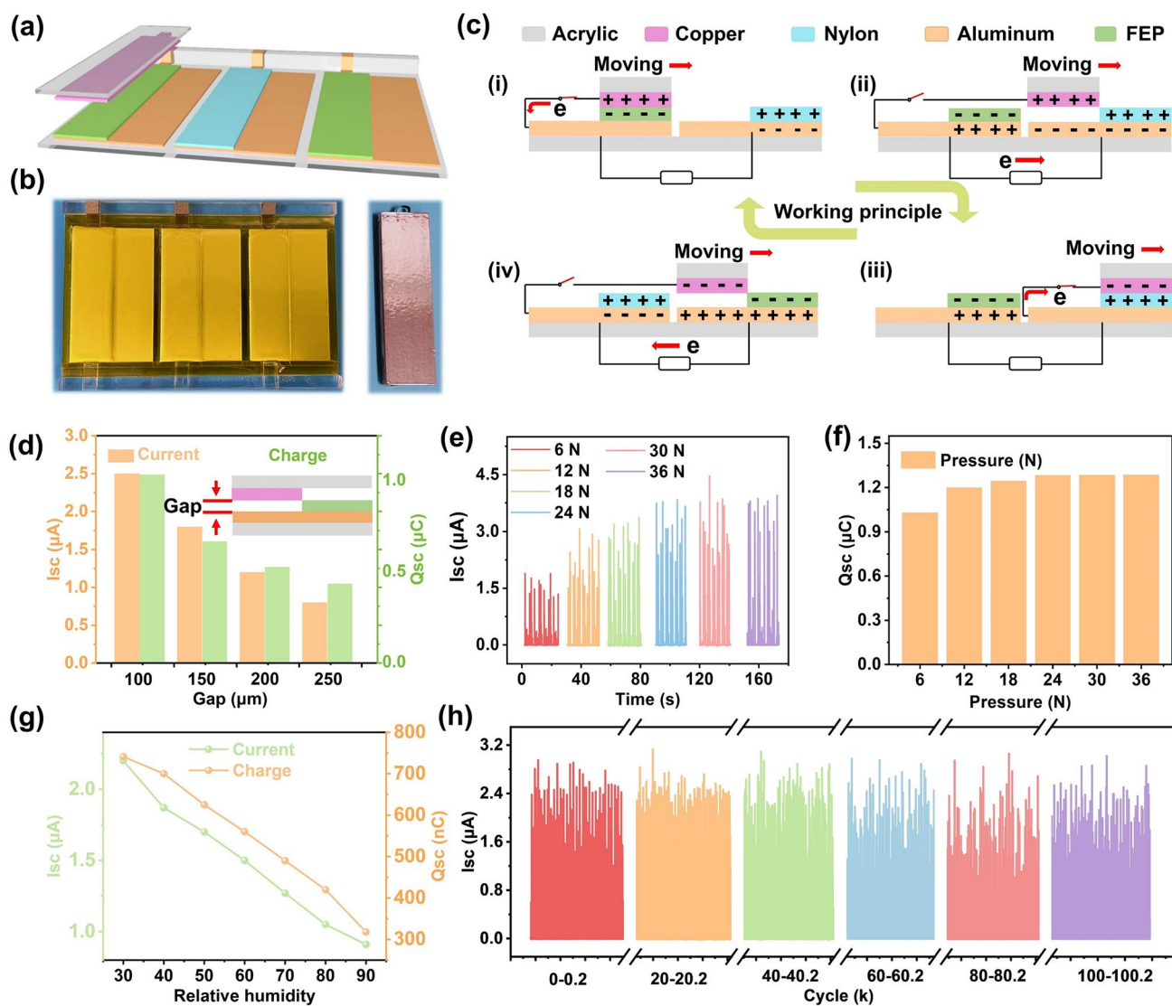
Fig. 2 The structure, working mechanism, and influence factors on the output performance of FS-PC-TENG. a, b 3D structural scheme and photographs of the FS-PC-TENG. c Schematic diagrams of working principle of the device. The basic short-circuit current and charge output of the FS-PC-TENG at d different air gaps, e, f different contact force, g different humidity. h The stability and durability of the FS-PC-TENG
