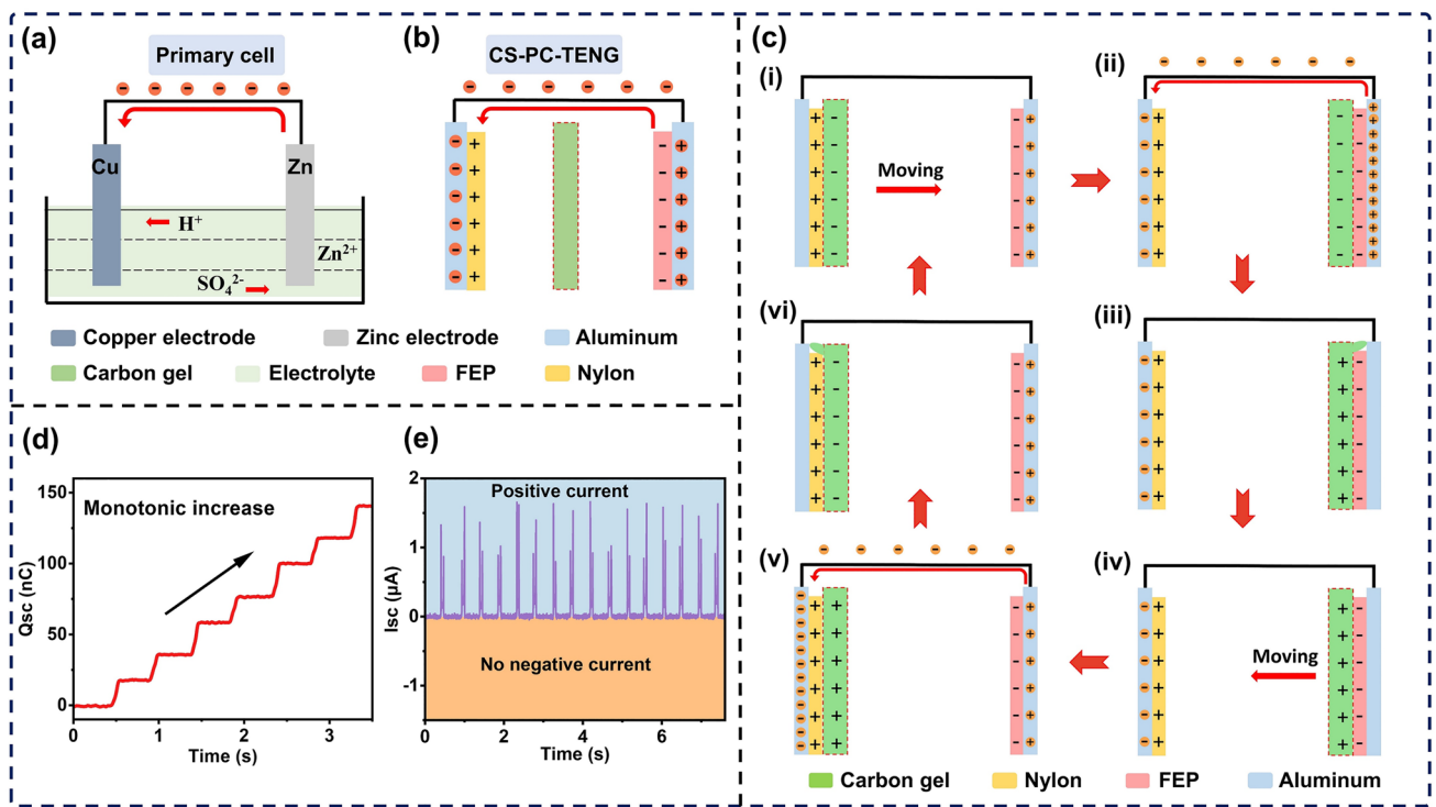
Fig. 1 The structural comparison of primary cell and the CS-PC-TENG, and working mechanism of the CS-PC-TENG. a Basic structure of the Zn/Cu primary cell. b Basic structure of the CS-PC-TENG. c Schematic diagrams of the working principle of the CS-PC-TENG. d, e The basic output charge and current of the CS-PC-TENG
