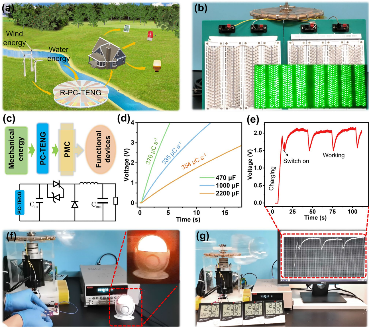
Fig. 4 Application of the R-PC-TENG powering different electronic devices. a The application scenario proposed for the R-PC-TENG. b Demonstration of directly powering 944 LEDs at 60 rpm. c System diagram and circuit diagram of the self-powered system for powering electronics with power management. d Voltage curves of charging 470, 1000, and 2200 \mu\text{F} capacitors by using R-PC-TENG device at rotational speed of 60 rpm. f Charging 2.2 mF capacitor while powering an infrared transmitting module under the driven of wind. e, g Charging 470 \mu\text{F} capacitor while powering four hydro-thermometers by wind energy
