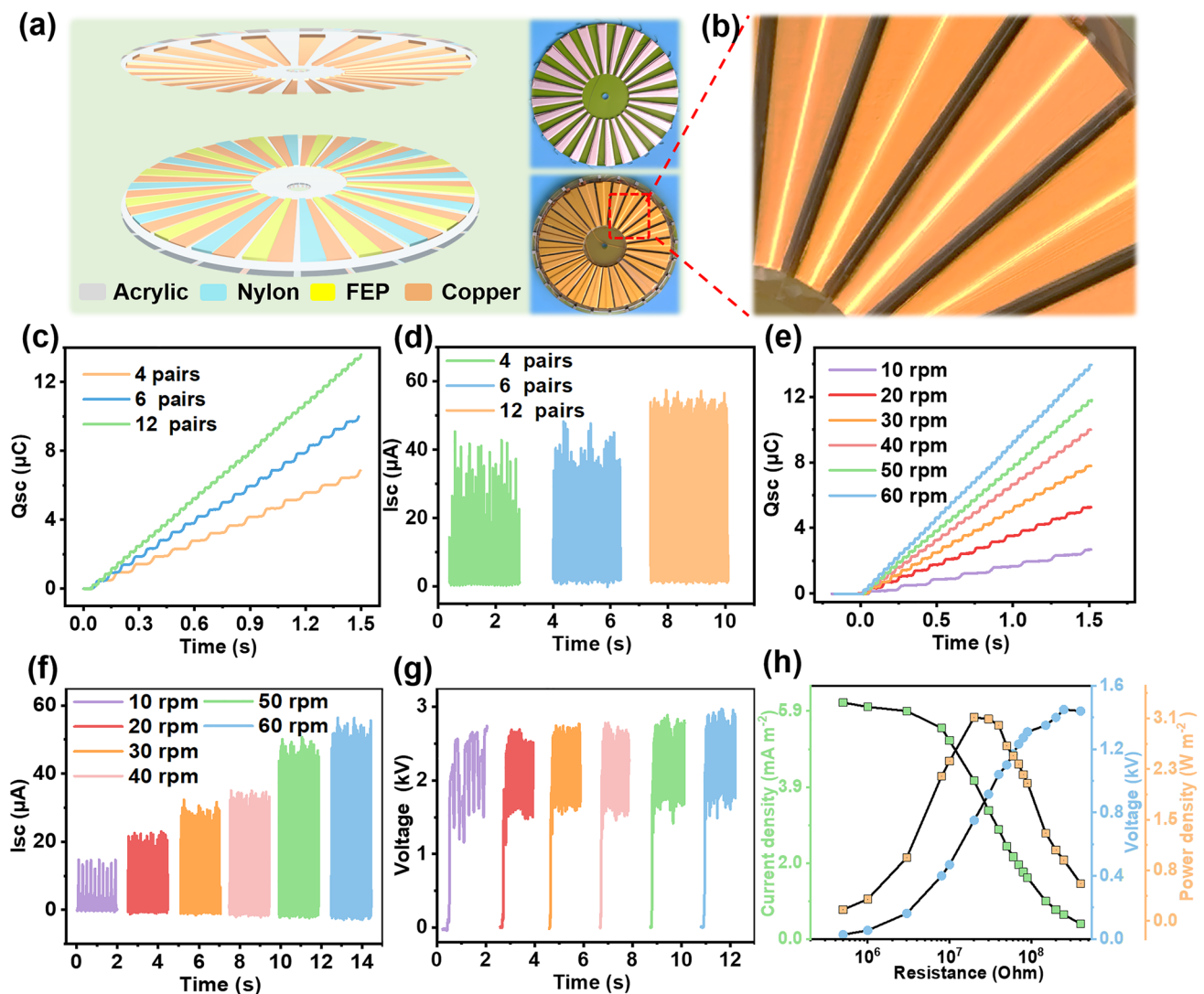
Fig. 3 The structure and performance of the R-PC-TENG. a 3D structural schematic of the R-PC-TENG device, and photographs of rotator and stator parts. b Partial enlarged detail of stator. c, d Transfer charge ( Q_{sc} ) and short-circuit current ( I_{sc} ) of R-PC-TENG with different pair of electrodes. e–g Transferred charge ( Q_{sc} ), short-circuit current ( I_{sc} ), and open-circuit voltage of the R-PC-TENG at different rotational speeds. h Evaluation of matching impedance and output power of the R-PC-TENG at rotational speed of 60 rpm
