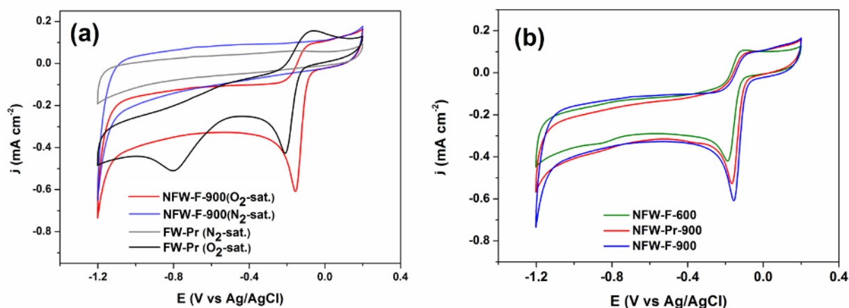
Figure 4. a) CVs of FW-Pr and NFW-F-900 in N_2/O_2 -saturated 0.1 M KOH, b) CVs of N-FWCNTs in O_2 -saturated 0.1 M KOH; at a 10 \text{ mVs}^{-1} scan rate.
