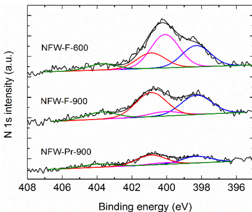
Figure 3. Deconvolution of N 1s XPS spectra of the NFW-F-600, NFW-F-900, and NFW-Pr-900 samples. The peaks are color-coded as pyridinic-N (blue), pyrrolic-N (magenta), graphitic-N (red), pyridinic N-oxide (green).
