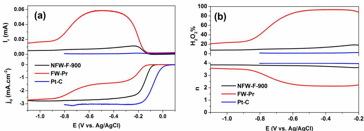
Figure 7. a) Disk and Pt-ring current density, b) \text{H}_2\text{O}_2\% and number of transferred electrons, for FW-Pr, NFW-F-900 and Pt-C; 5 \text{ mV s}^{-1} scan rate and 400 rpm in \text{O}_2 -saturated 0.1 M KOH.
