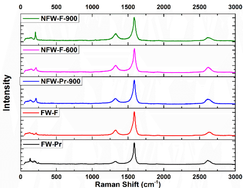
Figure 2. Raman spectra of the FW-Pr, FW-F, NFW-900, NFW-F-600 and NFW-F-900 samples.
