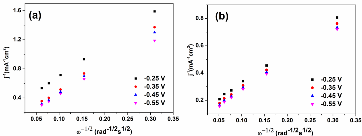
Figure 6. Koutecky-Levich plots for oxygen reduction on a) FW-Pr and b) NFW-F-900 in 0.1 M KOH. Data derived from Figure 5a.
