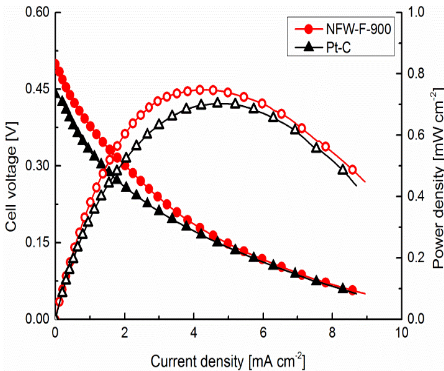
Figure 9. Polarization curves and power densities of the NFW-F-900 and Pt-C catalysts in a fuel cell test.
