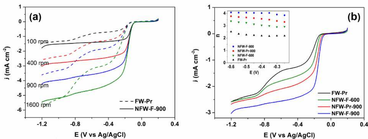
Figure 5. a) LSV of FW-Pr and NFW-F-900 at rotation rates from 100 to 1600 rpm, b) LSV of N-FWCNTs at 400 rpm (in O 2 -saturated 0.1 M KOH at 5 mVs -1 scan rate), inset: electron transfer number at different potential derived from K-L plots.
