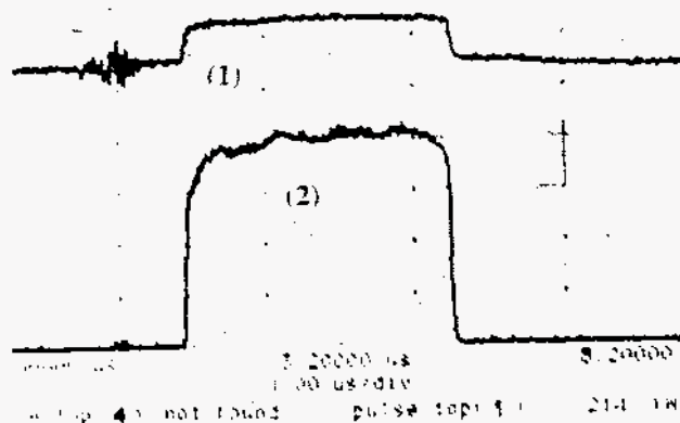
Figure 5: Oscilloscope waveforms showing: (1) forward power, (2) reflected power with a pulse width of 3.3 \mu s. Vertical scales are different in (1) and (2).
