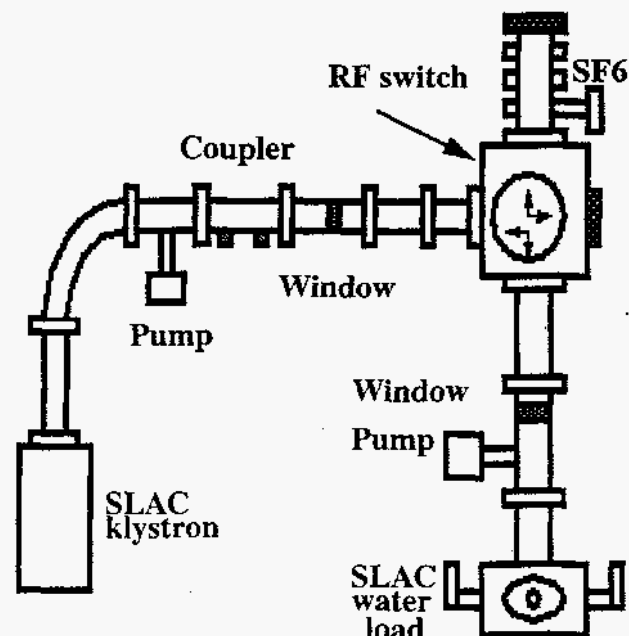
Figure 1: Schematic layout of the rf pressurized waveguide switch test.
