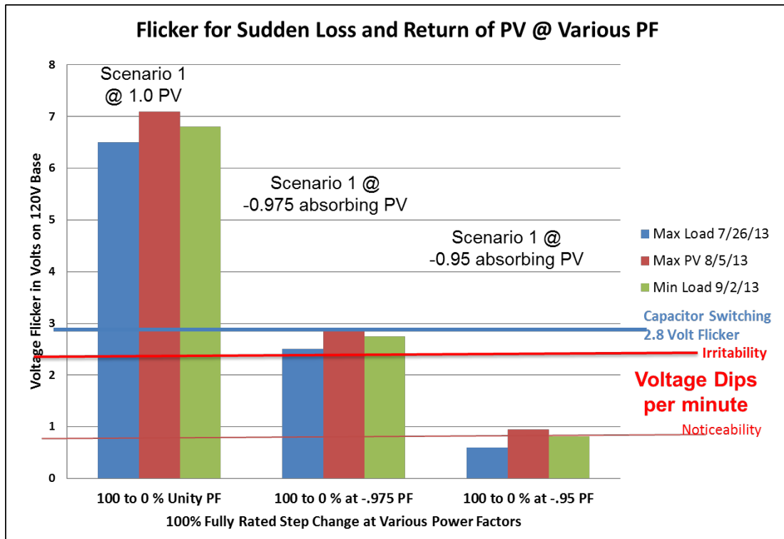
Figure 4.1. Porterville example study results—flicker associated with sudden loss and return of rated PV at the POI compared to the fixed absorbing power factor
