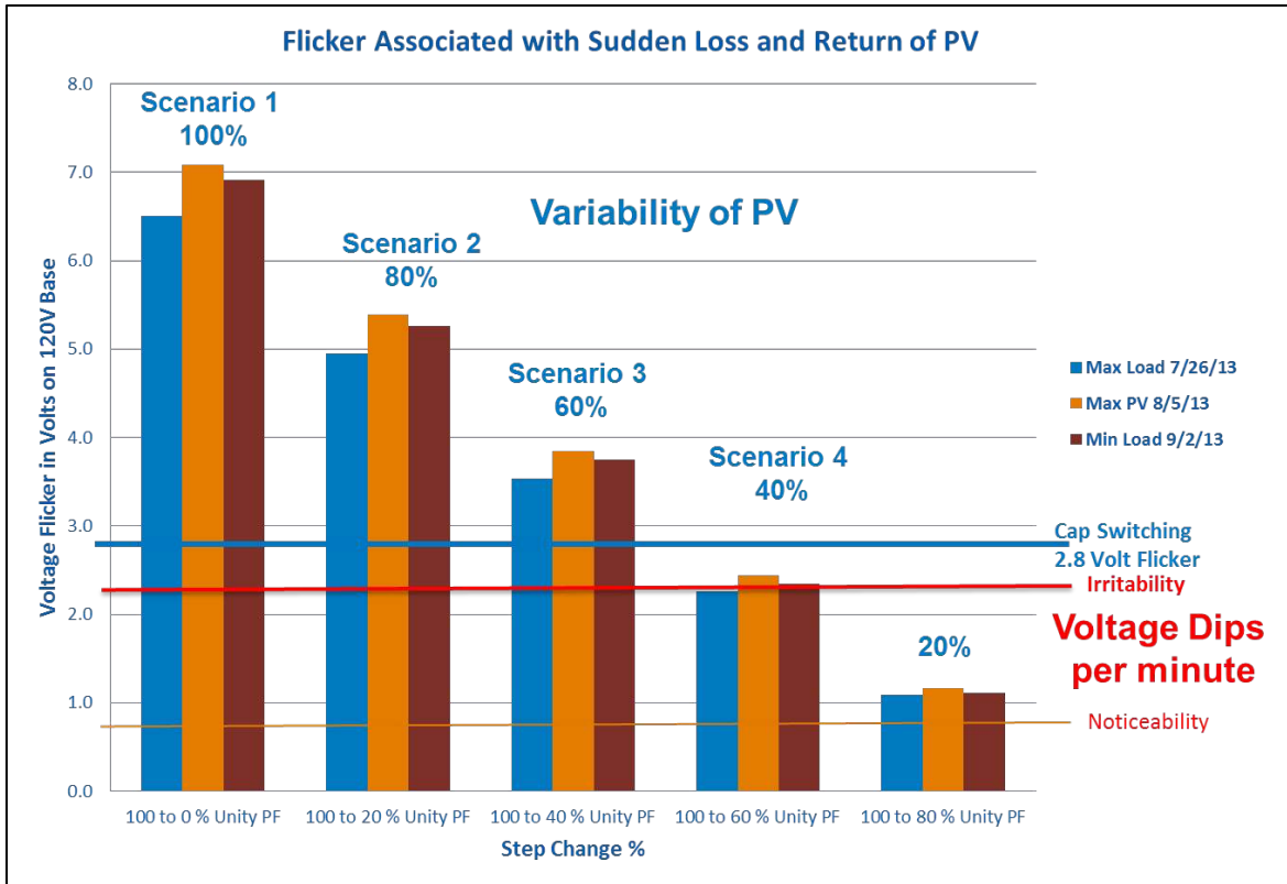
Figure 3.13. Porterville example study results—flicker associated with sudden loss and return of rated PV at POI
