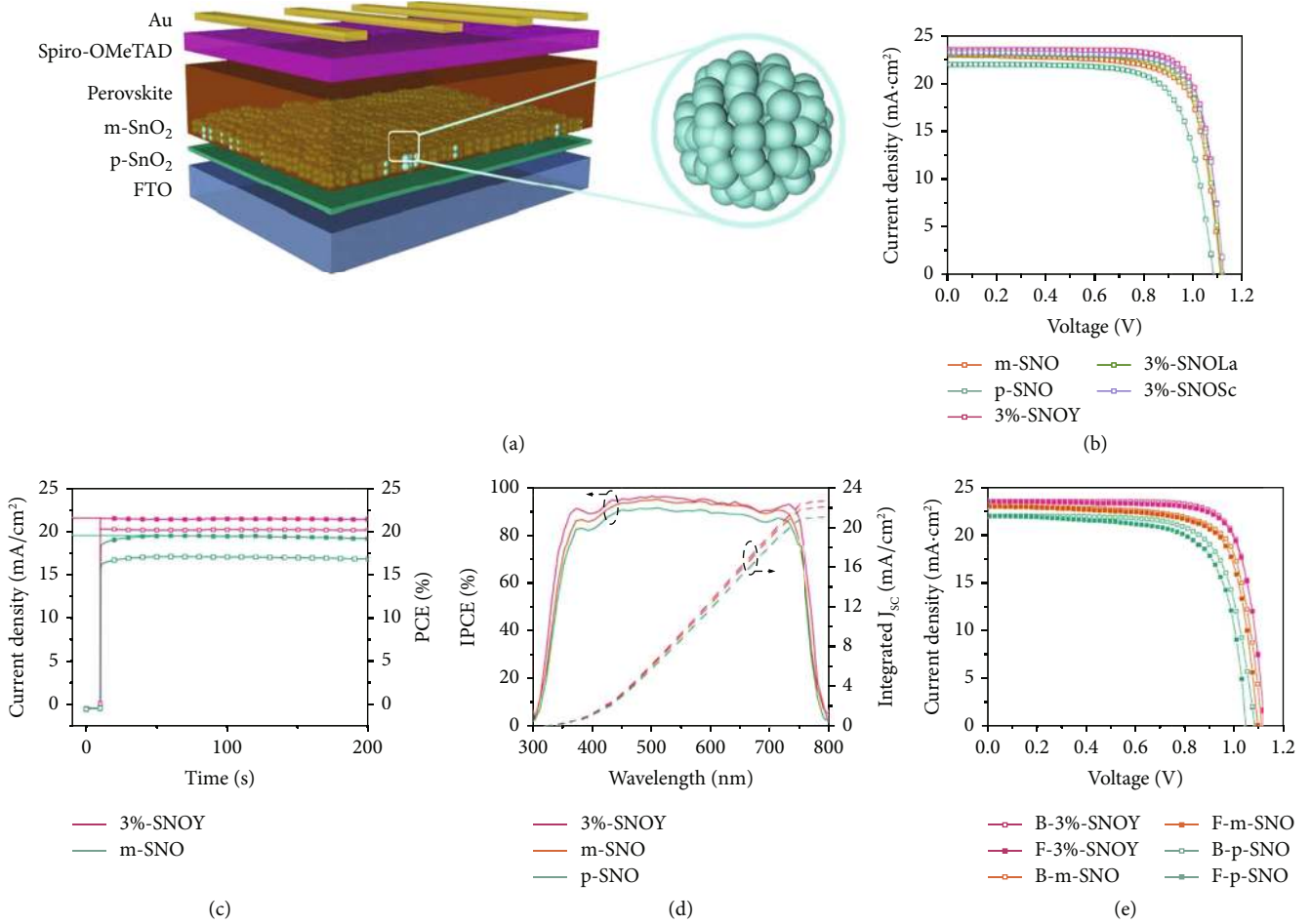
FIGURE 5: (a) Schematic device structure. (b) J - V curves of the PSCs with different \text{SnO}_2 . (c) Steady-state output of J_{\text{sc}} and PCE for m-SNO and 3%-SNOY devices. (d) IPCE spectra of the PSCs with different \text{SnO}_2 . (e) J - V curves of the PSCs with different \text{SnO}_2 under backward and forward scanning.
