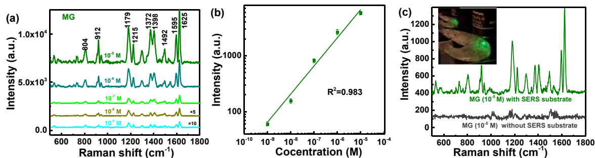
Figure 7: (a) Raman spectra of MG on the particle-in-multiscale 3D substrate (PDMS)/grating/zinc oxide nano spikes (ZnO NSs)/silver nanoparticles (Ag NPs) substrates. (b) Calibration curve of Raman intensity at 1625 \text{cm}^{-1} versus the concentration of MG. (c) Raman spectra of MG on the surface of shrimp.
