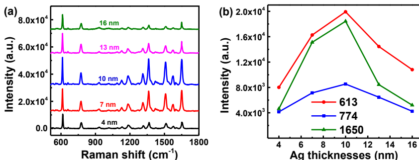
Figure 3: (a) Raman spectra of R6G with a concentration of 10^{-6} M on the particle-in-multiscale 3D substrate (PDMS)/grating/zinc oxide nano spikes (ZnO NSs)/silver nanoparticles (Ag NPs) substrates with different deposition thicknesses of Ag. (b) Corresponding Raman intensity of the peaks at 613, 774, and 1650 \text{cm}^{-1} .
