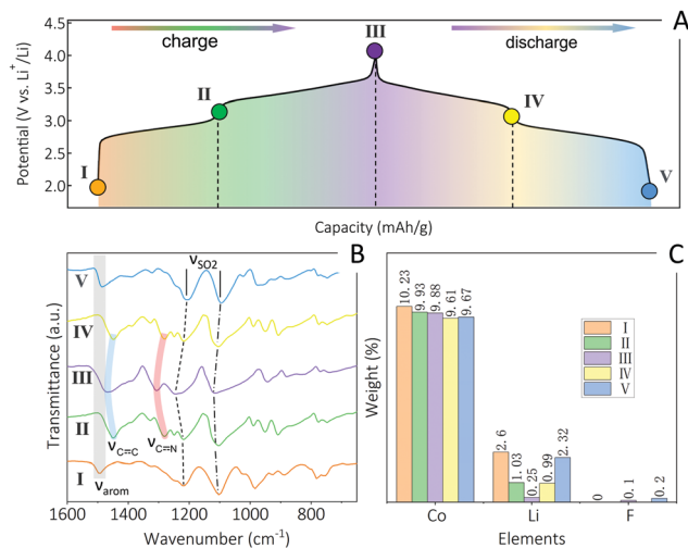
Fig. 5 Ex situ analysis of redox in Li_2 -Co-PTtSA. (A) The galvanostatic charge–discharge curve of with selected different dilithiation/lithiation states, and the five points marked represent various charge/discharge states of Li_2 -Co-PTtSA electrode: pristine (I), one electron half-charged (II), two electron full-charged (III), one electron half-discharged (IV) and two electron full-discharged (V). The corresponding ex situ FTIR spectra (B) and ex situ elemental analysis results (C).
