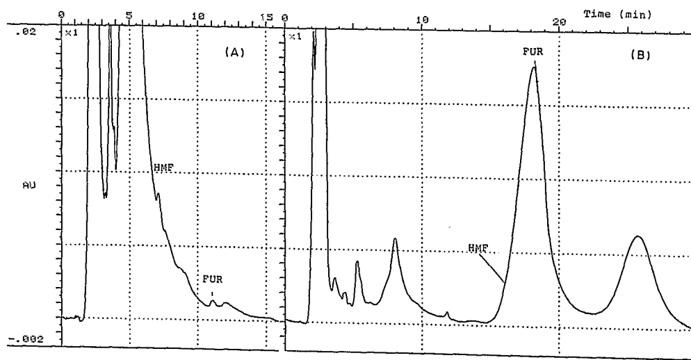
Figure 1 Typical chromatograms of hydroxymethylfurfural and furfural in juice concentrate. Column: Spherisorb ODS-2, 250 × 4.6 mm I.D., 3 µm. Flow rate: 1 ml/min. Temperature: 25 °C. Mobile phase: (A) Water/Acetonitrile (92 : 8). (B) Water/Tetrahydrofuran (99.7 : 0.3).
