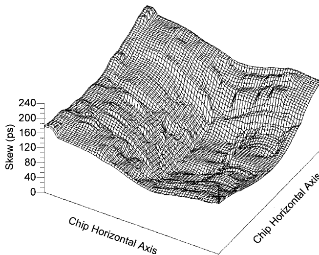
Fig. 14. 21064 clock skew.
