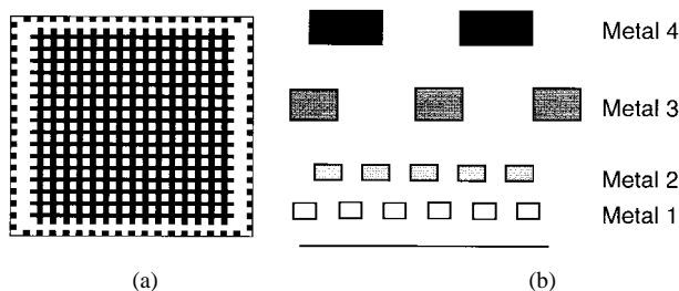
Fig. 11. (a) 21164 metal layers and (b) power distribution.
