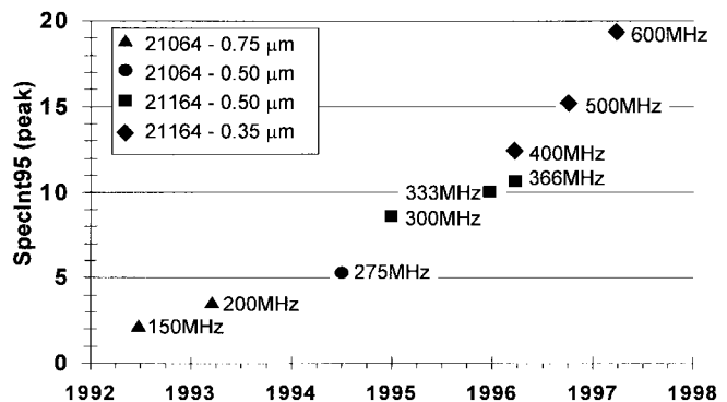
Fig. 1. Alpha performance versus time.
