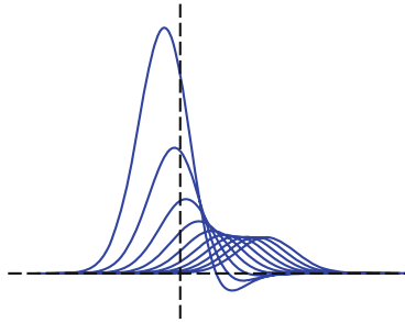
Fig. 3. Bias corrected kernel functions using the linear correction approach near a boundary (dashed line).
