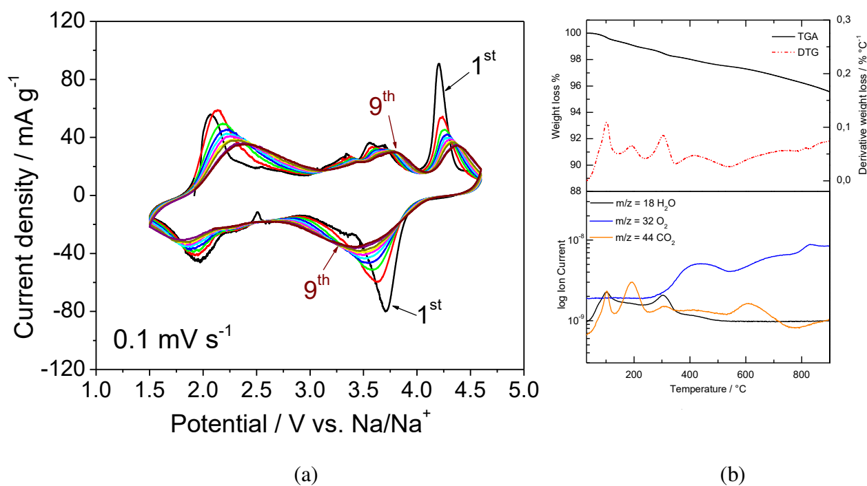
Figure 3. (a) Cyclic voltammogram of \text{Na}_{0.5}[\text{Ni}_{0.23}\text{Fe}_{0.13}\text{Mn}_{0.63}]\text{O}_2 performed at a scan rate of 0.1 \text{ mV s}^{-1} in the 4.6V-1.5V (vs Na/Na + ) voltage range at 20^\circ\text{C} \pm 2^\circ\text{C} ; (b) TGA-MS results for the rinsed material under He flux performed with a heating rate of 10K/min.
