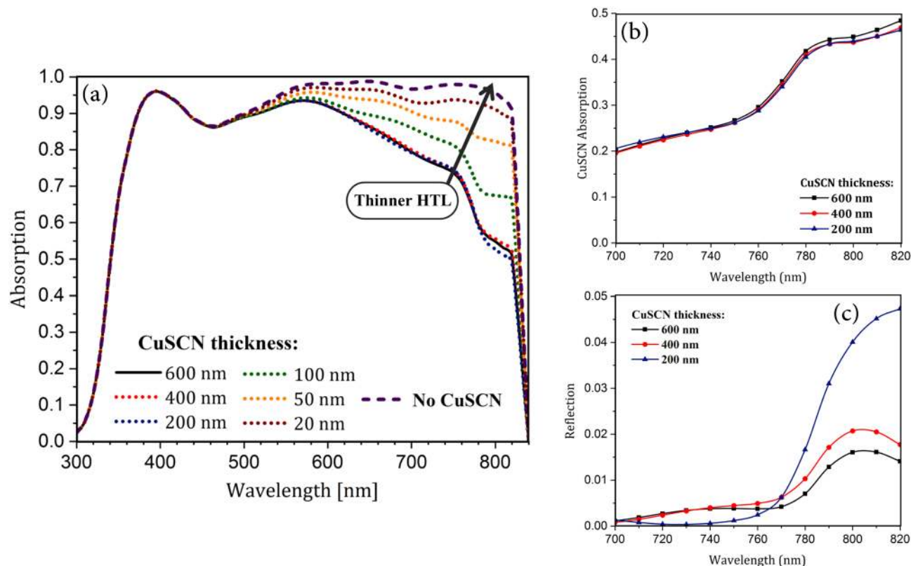
Fig. 7. Normalized absorption and reflection of the convex nanostructured PSC (structure (IV)) with different thicknesses of HTL. (a) Normalized perovskite absorption of Str (IV) with the HTL thicknesses of 600, 400, 200, 100, 50, and 20 nm. (b) Normalized CuSCN absorption, and (c) normalized reflection from Str (IV) with the HTL thicknesses of 600, 400, and 200 nm.
