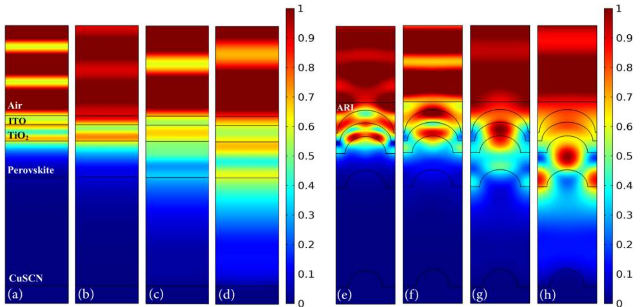
Fig. 6. Profile of normalized electric field for the planar and proposed structures. (a,e) At the wavelength of 390 nm, (b,f) at 480 nm, (c,g) at 630 nm, and (d,h) at 800 nm.
