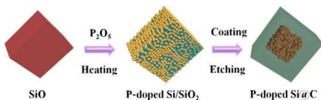
Figure 2 The fabrication procedure of P-doped Si@C material.
