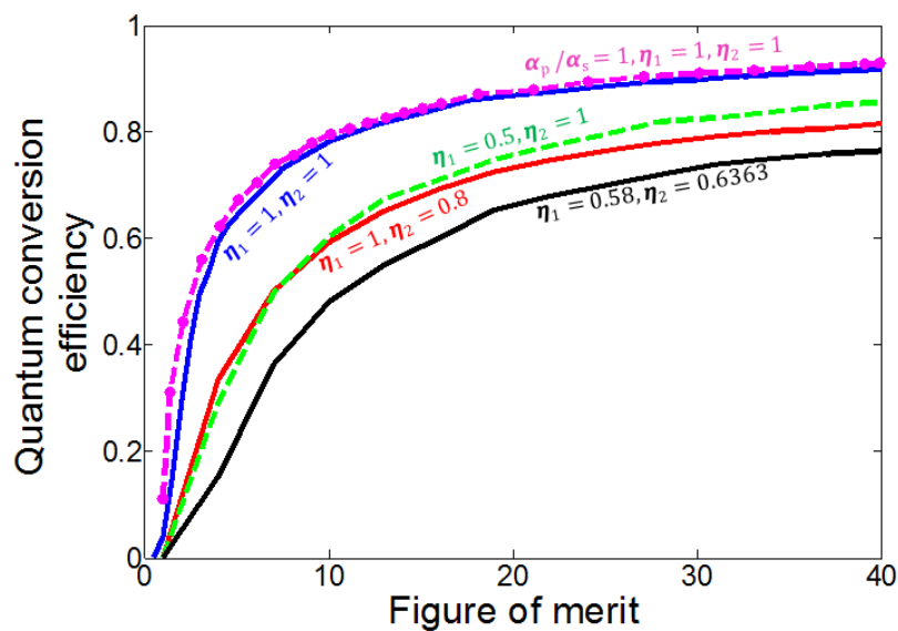
Figure 11. Simulated curves of quantum conversion efficiency vs. figure of merit ( p_0 = g_R I_{p0} / \alpha_s ) for optimized out-coupling and fiber length for different re-launch efficiencies at out-coupling end ( \eta_1 ) and HR re-launch end ( \eta_2 ). Loss ratio \alpha_p/\alpha_s = 1.09 , except for the uppermost curve, which has a loss ratio of 1.
