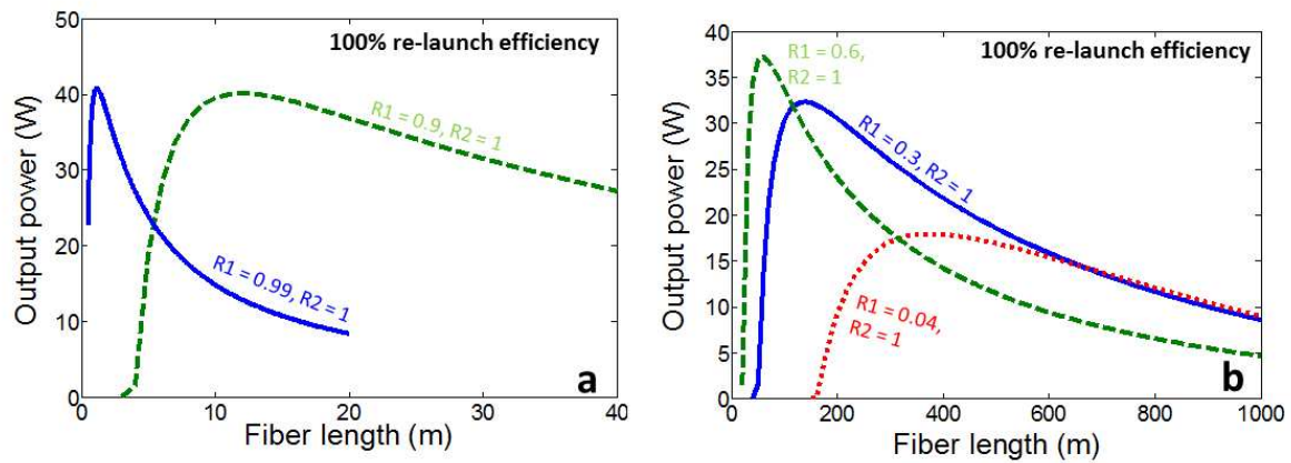
Figure 8. (a) Simulations of the output power vs. DCRF length at pump power of 65 W (launched) for out-coupling ratio (R1) of 0.9 and 0.99 and for 100% re-launch efficiencies for pump as well as Stokes wave in both ends of the cavity; (b) Simulations of the output power vs. DCRF length at pump power of 65 W (launched) for various out-coupling ratio (R1) and 100% re-launch efficiencies.
