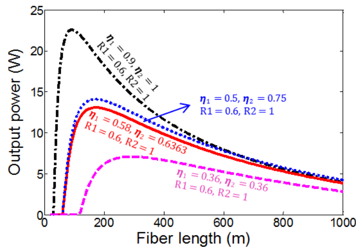
Figure 9. Simulation of output power vs. DCRF length at pump power of 65 W (launched) for different reflectivities of the output coupler (R1) and re-launch efficiencies ( \eta_1 corresponds to out-coupling end and \eta_2 corresponds to high reflectivity end ).
