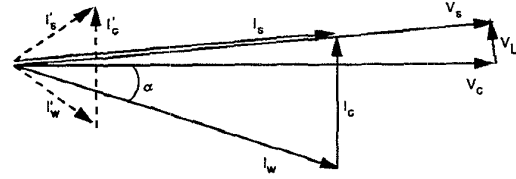
Fig. 6 Phasor diagram of a converter system
