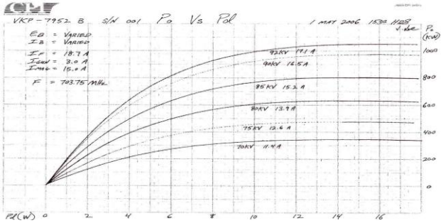
Fig. 6 This set of data was used to determine the amount of expected at a given beam Voltage
