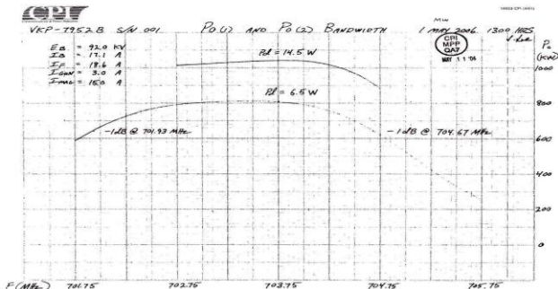
Fig. 7 Bandwidth at two different drive levels. This tube could also be designed with a greater bandwidth and a lower gain.
