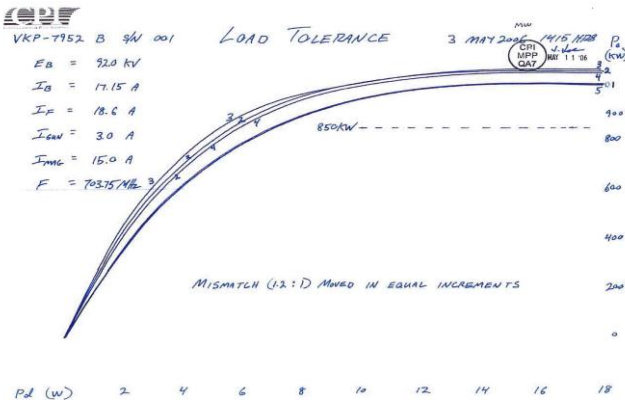
Fig. 8 Load tolerance was measured at the factory with calibrated mis-matches. It shows the effect on the output due to load VSWR
