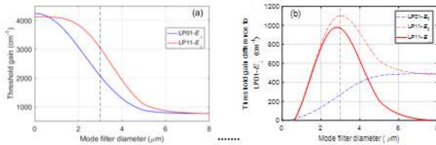
Fig. 3. Dependence of a) threshold gain for the transverse \text{LP01-}E_{\perp} and \text{LP11-}E_{\perp} modes and b) transverse and polarization mode discrimination (threshold gain differences) on mode filter (grating) diameter. The grating pitch, depth, and fill-factor is 120 nm, 59 nm, and 55%, respectively. The diameter of the oxide aperture is 5 \mu\text{m} .
