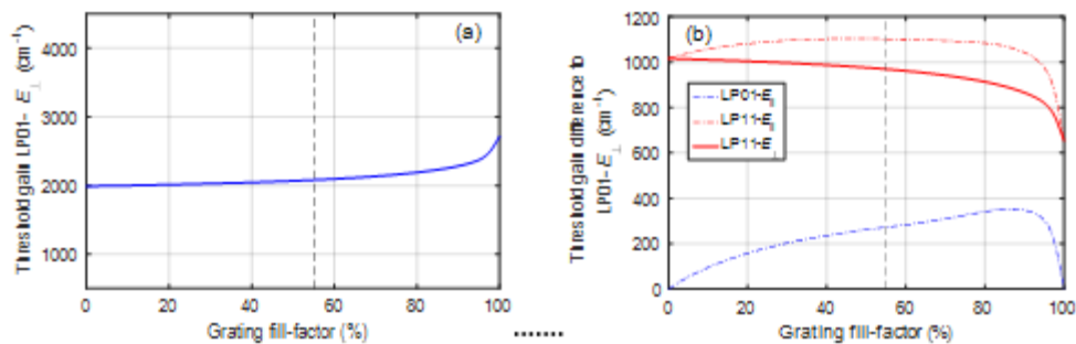
Fig. 4. Dependence of a) threshold gain for the fundamental transverse \text{LP01-}E_{\perp} mode and b) transverse and polarization mode discrimination (threshold gain differences) on grating fill-factor. The grating pitch and depth is 120 and 59 nm, respectively, and the oxide aperture and mode filter diameters are 5 and 3 \mu\text{m} , respectively.
