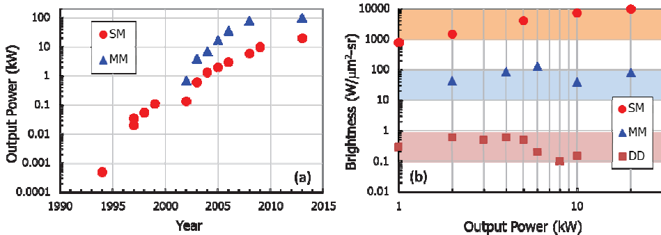
Fig. 13. (a) Power evolution with time and (b) brightness variation with power for single-mode (SM) and multimode (MM) Yb-doped cladding-pumped fiber lasers [direct diode (DD) is shown also for comparison 152 ].
