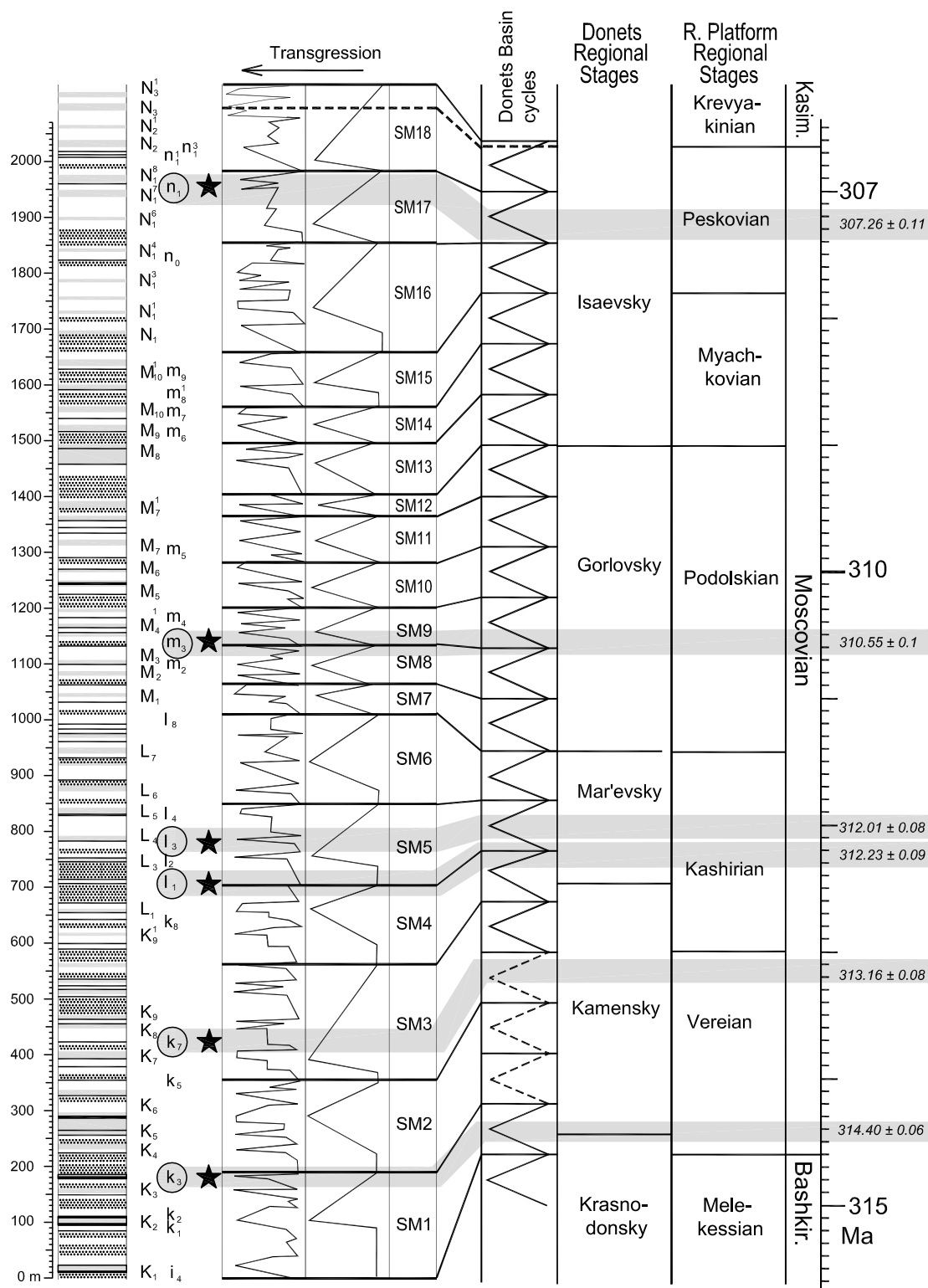
Figure 6. Lithostratigraphy and sequence stratigraphy through the Moscovian succession of the central exposed Donets Basin (modified from Izart et al. [1996, Figure 3]), with positions of six radiometric ages obtained in our study. Projection of stratal architecture onto a time linear scale constrained by ash bed ages reveals the consistent \sim 400 ka tempo of the fourth-order sequences of Izart et al. [1996]. Only a few high-frequency cycles in the lowermost Moscovian must be reinterpreted as fourth-order major transgressions to maintain consistency with the model. Tuning of these fourth-order sequences to the long eccentricity cycle allows calibration of the biostratigraphic record at a resolution of \sim 100 ka.
