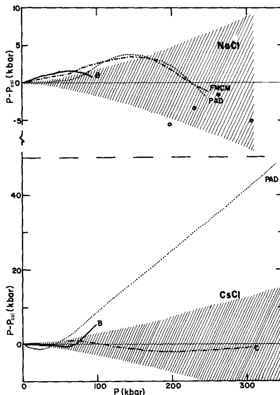
FIG. 3. Differences between the calculated pressure from the equation of state and measurements of Bridgman; B; Perez-Albuera and Drickamer; PAD; Fritz, Marsh, Carter, and McQueen; FMCM; Weaver, Takahashi, and Bassett; C; and Christian; C. See text for references. The diverging dashed lines indicate the uncertainty in the calculation resulting from uncertainties in the measured input parameters.
