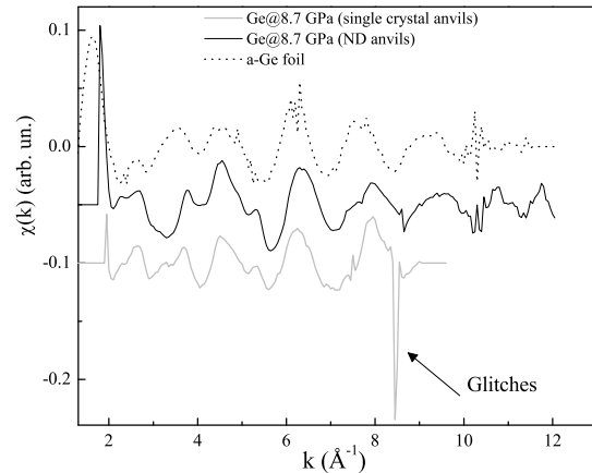
FIG. 1: EXAFS signal of Ge obtained with ND anvils (black line) and single crystal anvils (grey line). EXAFS function of standard amorphous Ge foil obtained without DAC (dot line). An offset was added to the EXAFS signals.
