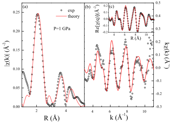
FIG. 4: Comparison between the experimental EXAFS spectrum collected with ND anvils at 1 GPa (dots) and the best-fit calculation (solid curve) using three Ge-Ge paths. Comparison is reported for the moduli of the Fourier transform (a) the extracted k\chi(k)\text{\AA}^{-1} signal (b), and for the real part of the back-transformed signal (c).
