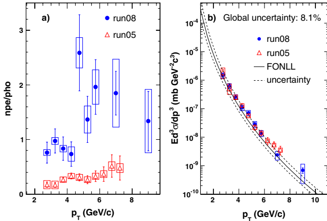
FIG. 15 (color online). (a) Ratio of nonphoton to photon electron yield from the Run2008 (closed circles) and the Run2005 (open triangles) analyses. (b) Invariant cross section for nonphoton electron production ( \frac{e^+ + e^-}{2} ) in p + p collisions from the Run2008 (closed circles) and the Run2005 (open triangles) analyses. The error bars and the boxes represent statistical and systematic uncertainty, respectively. The solid line is FONLL calculation and the dashed lines are the FONLL uncertainties [2].
