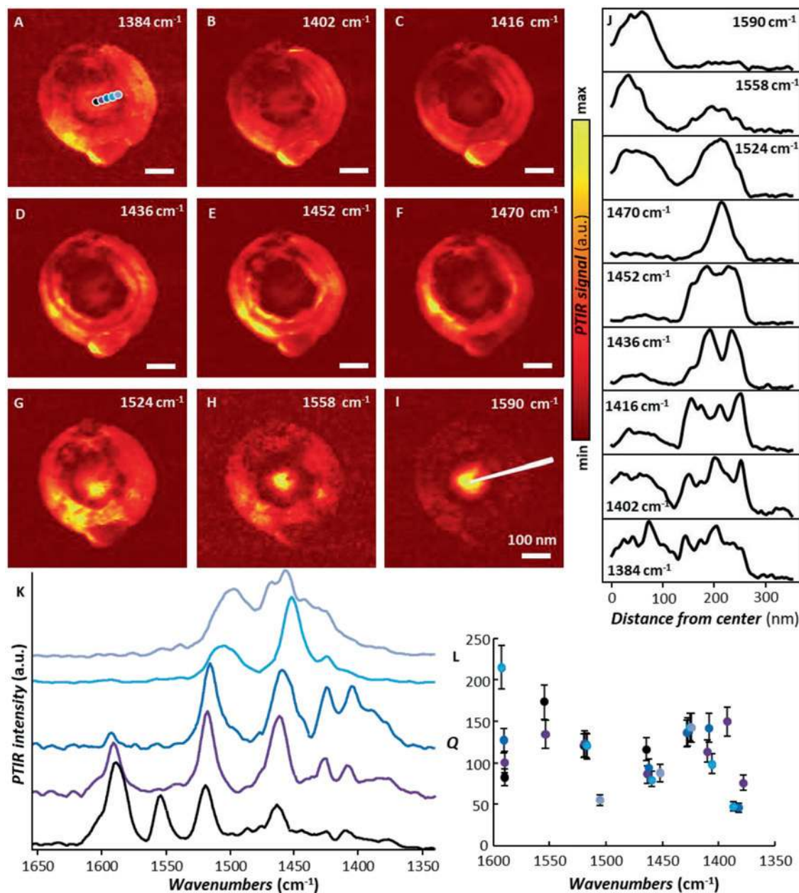
Figure 3: (A–I) Tapping-mode PTIR absorption maps for an hBN frustum of A_r = 1.16 \pm 0.03 . All images (3 and 7.5 nm pixel resolution in the horizontal and vertical directions respectively) were obtained with a scan rate of 0.6 Hz using probe-B. Scale bars are 100 nm. (J) Line cuts of the PTIR images along the direction indicated by the white line in panel-I. (K) Tapping-mode PTIR spectra obtained at the color-coded position in panel-A. The spectra are displayed in full scale with an offset for clarity. (L) Q-factors of the polariton resonances obtained from the color-coded spectra in panel-K. The error bars represent a single standard deviation in the determination of Q and mainly determined by the uncertainty of determining the peaks FWHM via the least square fitting the resonances with Lorentzian peak shapes.
