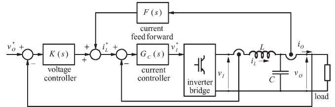
Fig. 3. Per-phase structure of conventional voltage control loop.
