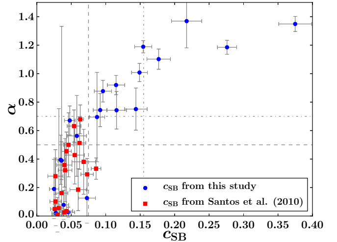
Figure 2. Correlation between \alpha and c_{\text{SB}} for the CCCP high- z clusters. Values for \alpha are from Vikhlinin et al. (2007). Values for c_{\text{SB}} with z < 0.5 are reported in this study. Values for c_{\text{SB}} with z \geq 0.5 are from Santos et al. (2010). The dashed lines correspond to the boundaries between noncool cores and moderate cool cores. The dash-dotted lines correspond to the boundaries between moderate cool cores and strong cool cores.
