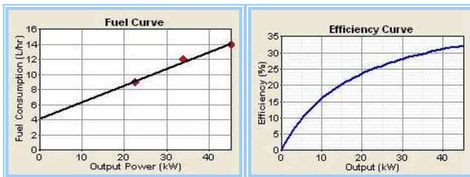
Fig. 2. Typical fuel consumption characteristics of diesel generator
