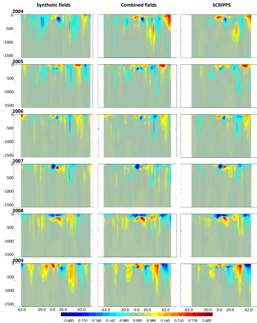
Fig. 11. Yearly zonal averages of the synthetic, combined and SCRIPPS temperatures as anomalies from the 2004 to 2009 periods (in °C). The latitudinal extents of each field are slightly different.
