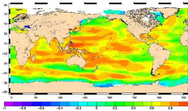
Fig. 1. Annual correlation coefficient between dynamic heights (DH) computed using a reference level at 1500 m depth and temperature ( T ) field at 100 m depth. The color scale ranges from -1 to 1 , every 0.1 .
