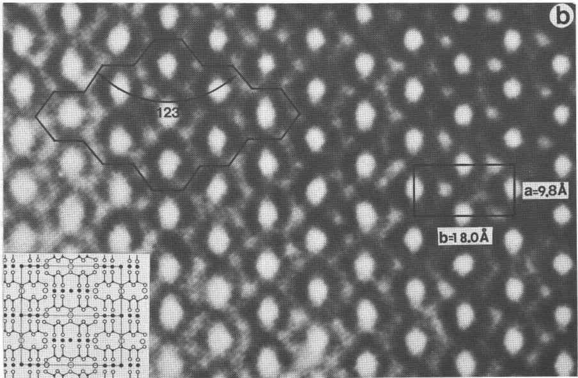
FIG. 11 a. High magnification structure image of an a - b section of orthoenstatite. The white regions correspond to the M_2 sites. A unit cell is outlined; the insert shows the orthoenstatite structure at the same scale as the electron image. Possible cleavage surfaces are sketched in the upper left. b. High magnification structure image of an a - b section of hornblende. The white regions correspond to the "A" sites. A unit cell is outlined; the insert shows the amphibole structure at the same scale as the structure image. Possible cleavage surfaces are sketched in the upper left.
