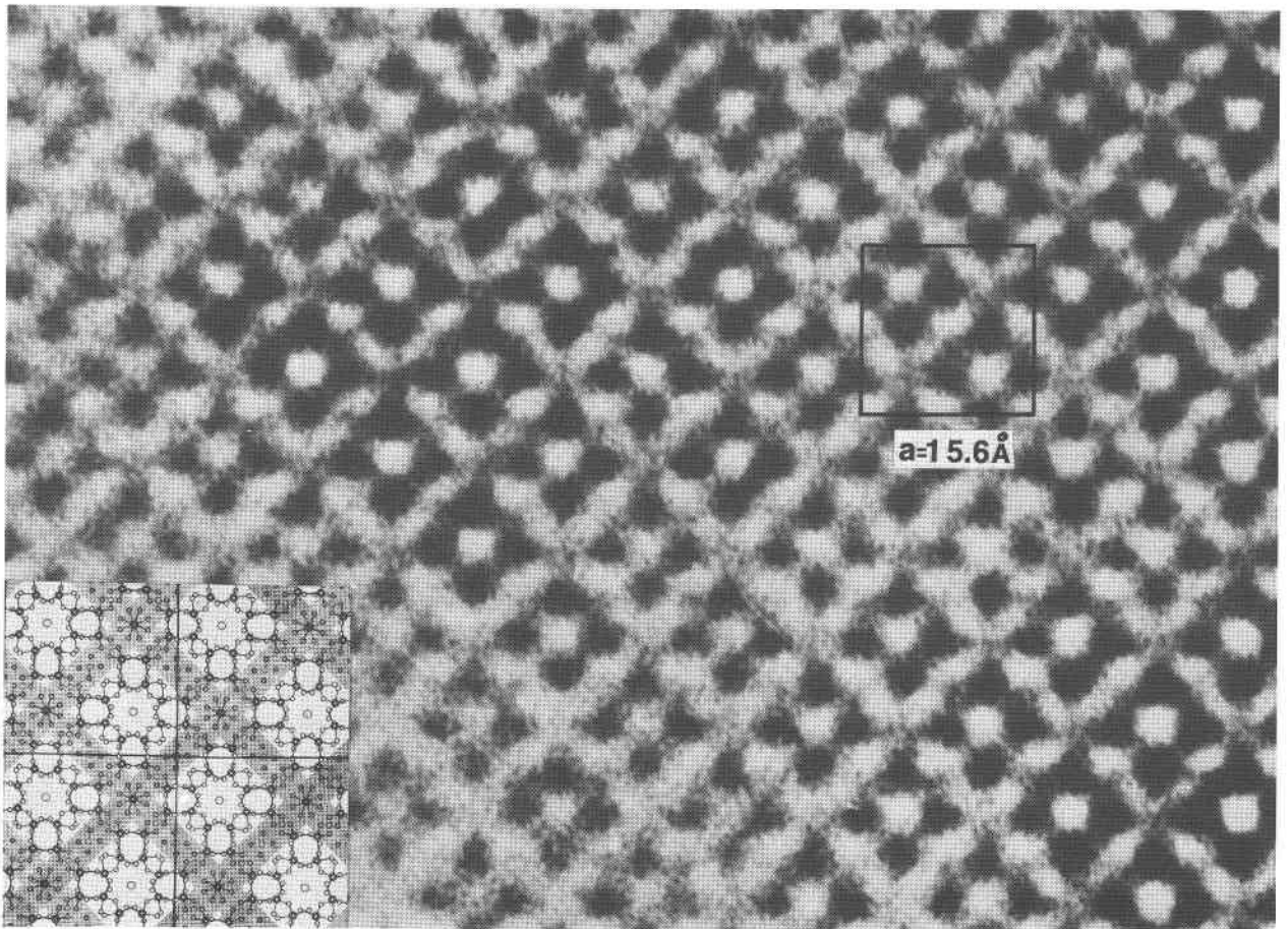
FIG. 8. High magnification structure image of idocrase showing a section perpendicular to c . A unit cell is outlined, and the insert shows several cells from Figure 7 at the same scale as the structure image. The projected zones containing Al sites and the "R" and "T" sites have been shaded slightly.
