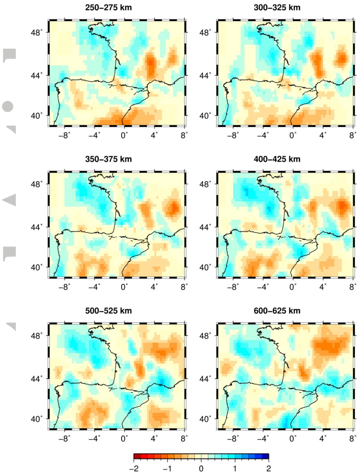
Figure 11. (Continued) Map views of the model for P velocity anomalies at 250, 300, 350, 400, 500, and 600 km depth.
