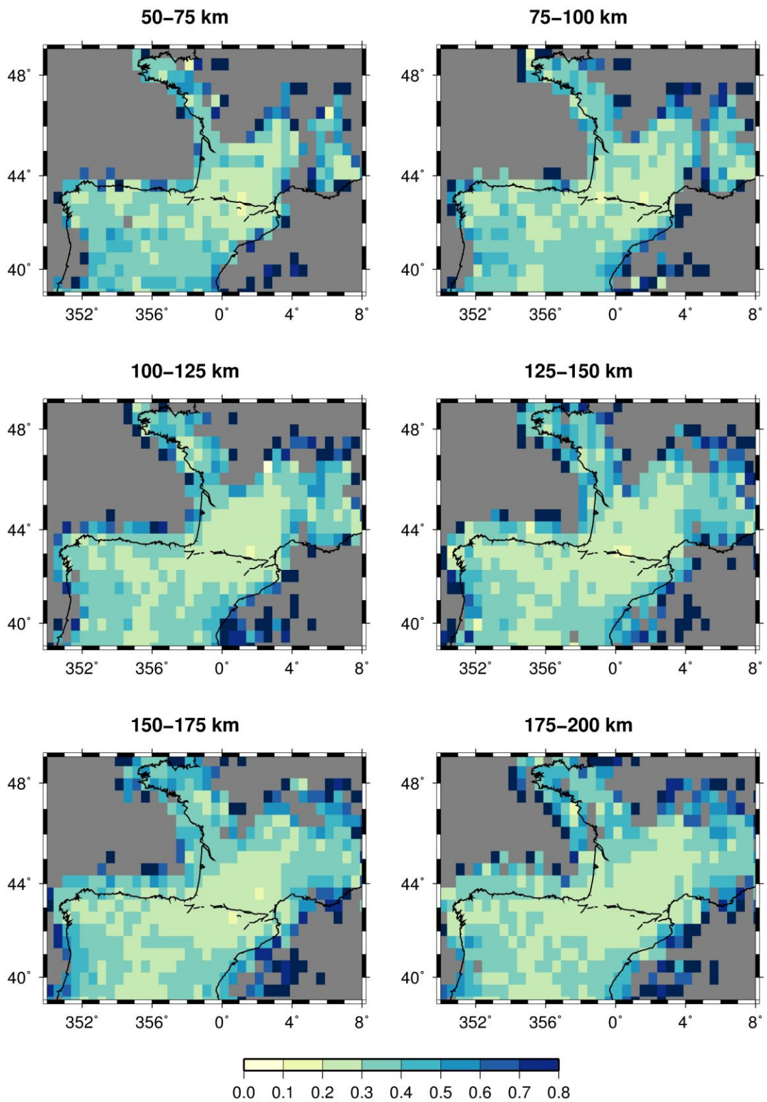
Figure 8. Lateral resolution (in degrees) in the tomographic grid, from 50 km to 200 km depth.
