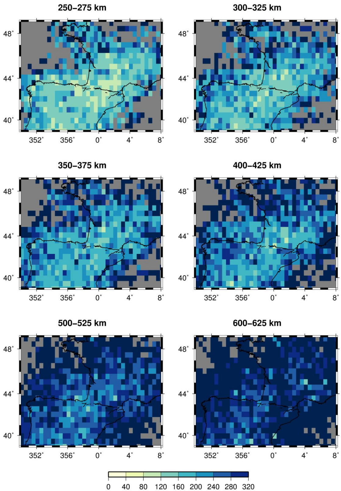
Figure 9. (Continued) Vertical resolution (in km) in the tomographic grid, from 250 km to 625 km depth.
