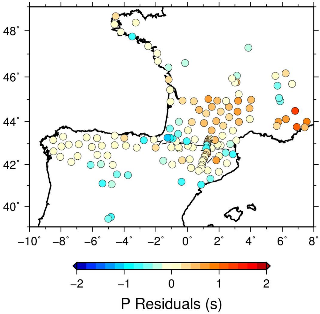
Figure 4. Map of of P residuals for the 11/08/2012 Zagros event.
