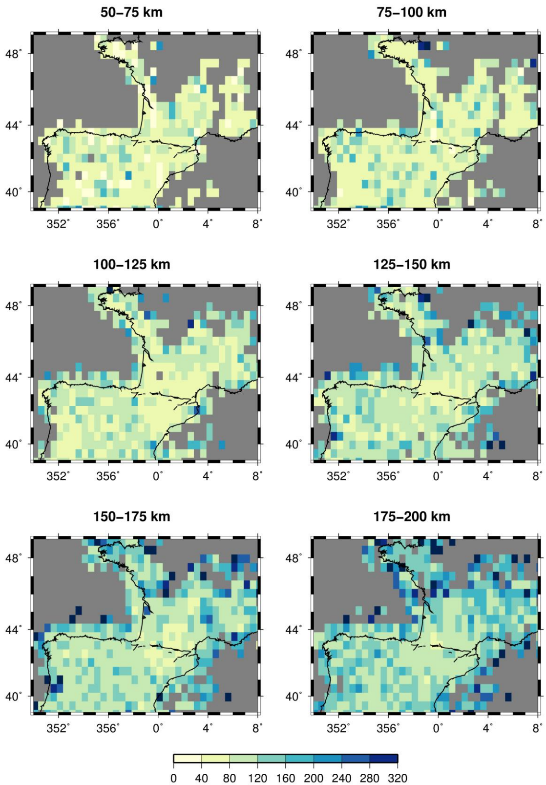
Figure 9. Vertical resolution (in km) in the tomographic grid, from 50 km to 200 km depth.
