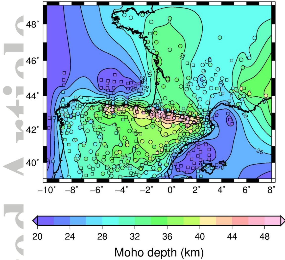
Figure 6. Map of crustal thickness. This map was obtained by interpolating the crustal thicknesses obtained from receiver functions (circles) and seismic reflection/refraction profiles (squares).
