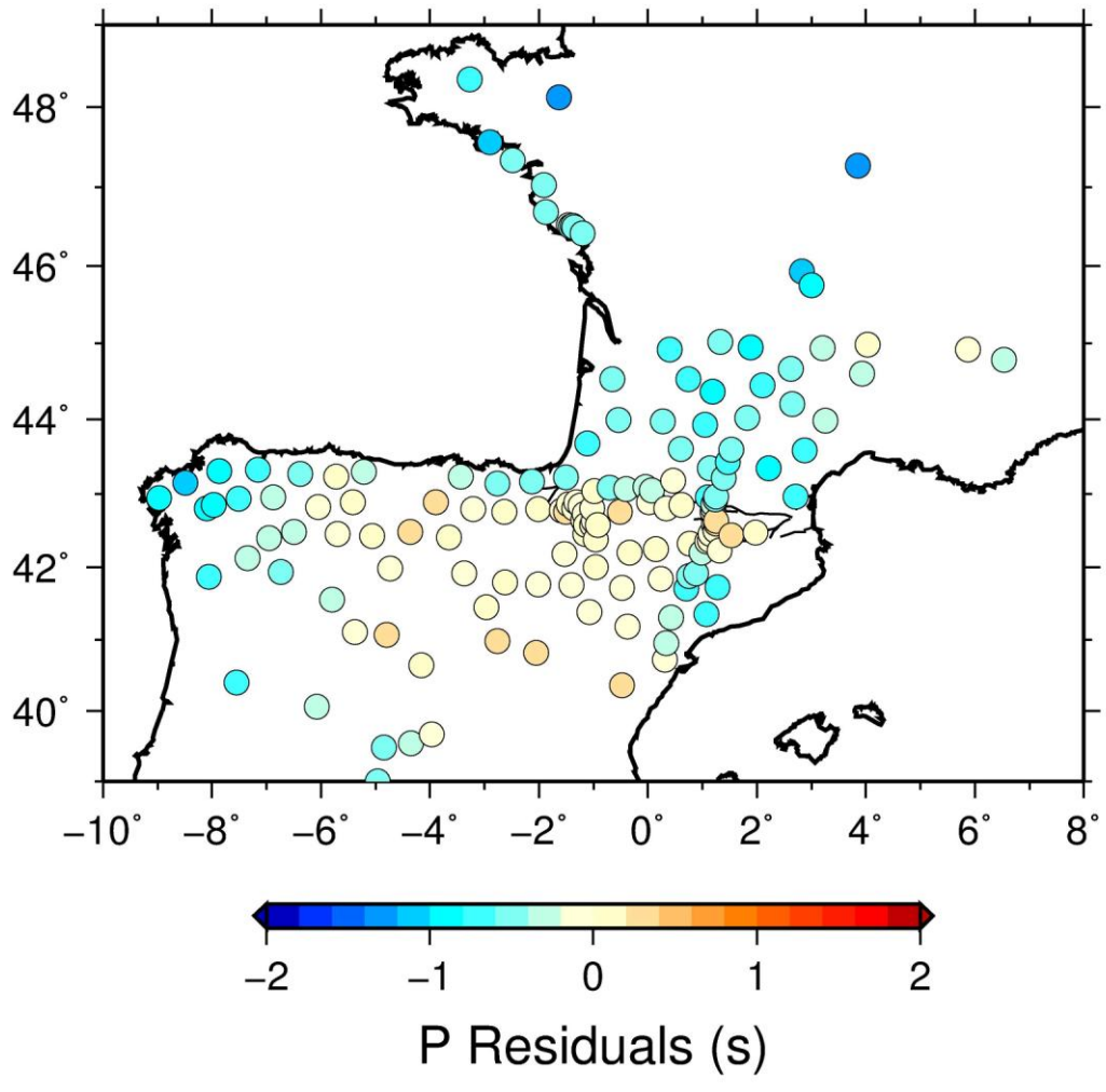
Figure 3. Map of P residuals for the 17/11/2011 Ecuador event.
