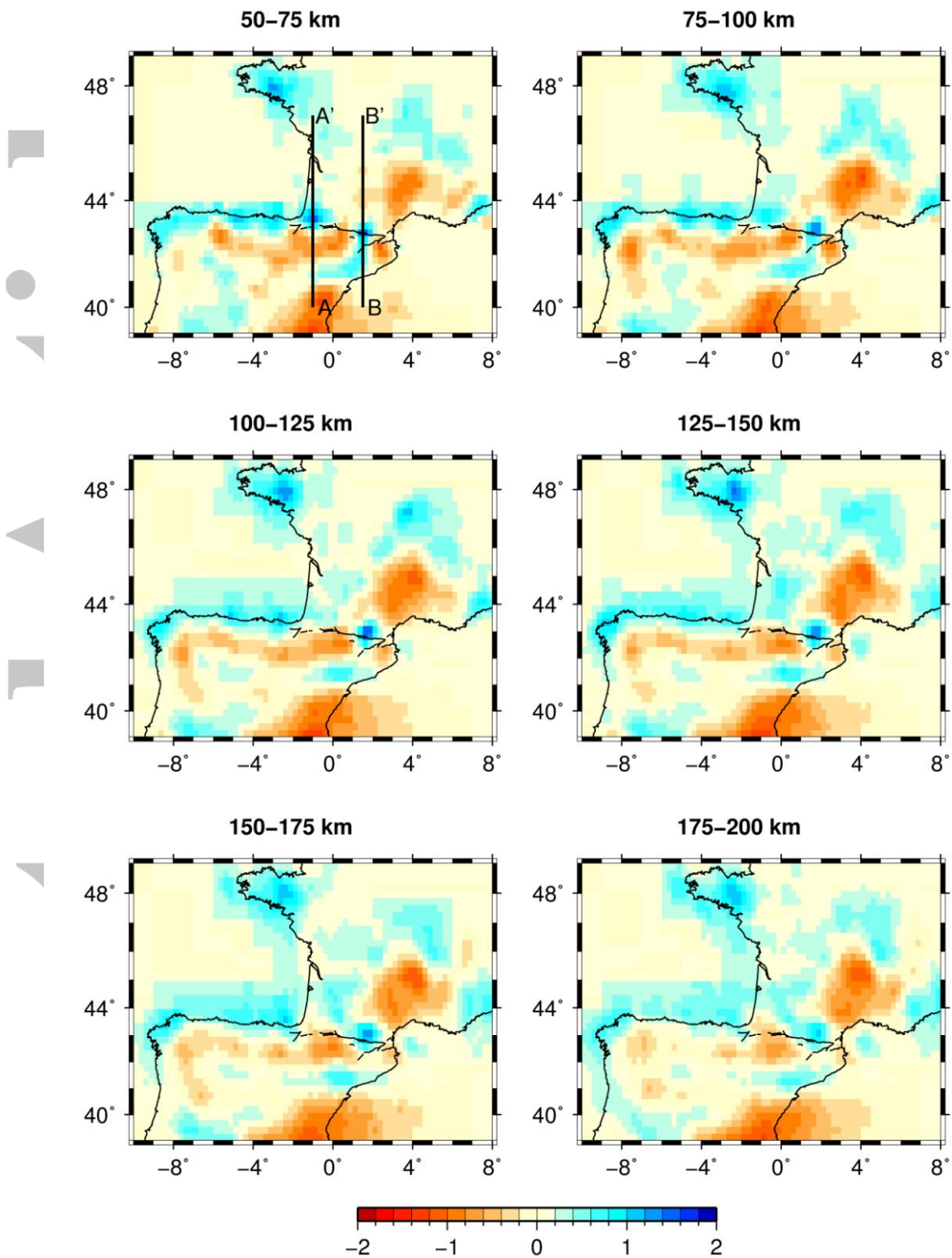
Figure 10. Map views of the P velocity model obtained without crustal corrections at 50, 75, 100, 125, 150, and 175 km depth. The color scale, in percents with respect to ak135 reference Earth model, is the same in all the plots.
