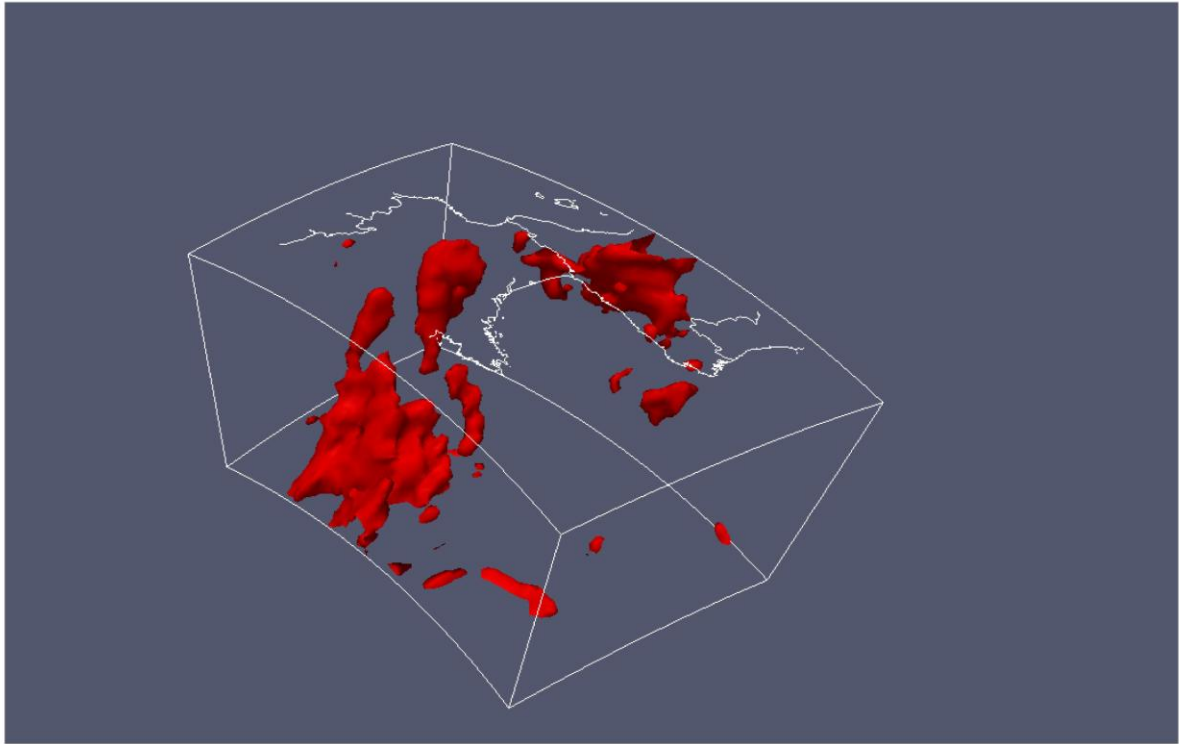
Figure 13. 3-D view of the isocontour corresponding to a perturbation of -0.75 % of the P velocity. The bottom of the box is at 900 km depth. The broad low velocity anomaly in the transition zone is not connected from the shallow asthenospheric anomaly beneath the Massif Central.
