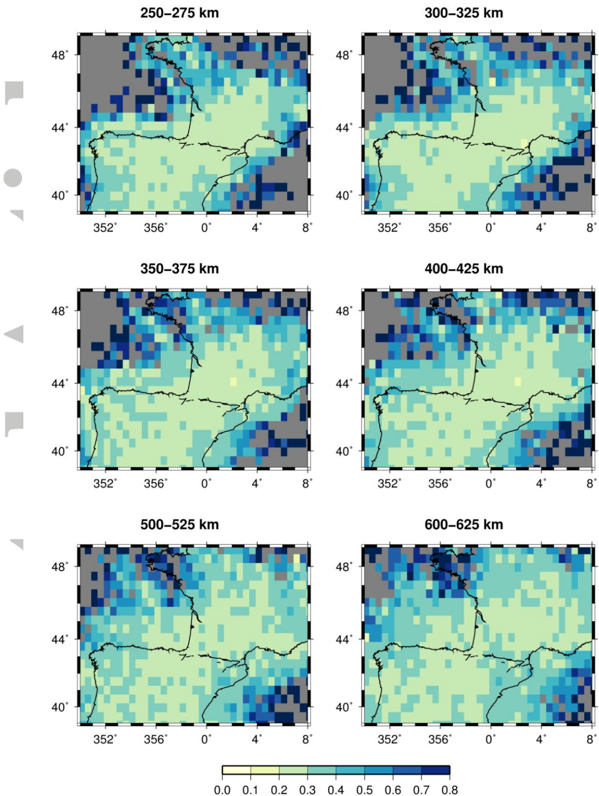
Figure 8. (Continued) Lateral resolution (in degrees) in the tomographic grid, from 250 km to 625 km depth.
