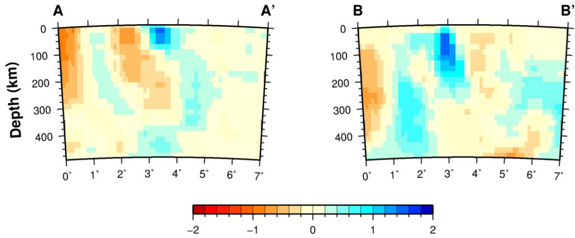
Figure 12. N-S vertical cross-sections along longitudes 1.0^{\circ} W (left) and 1.5^{\circ} E (right). The geometries of the two cross-sections are shown in Figure 11.
