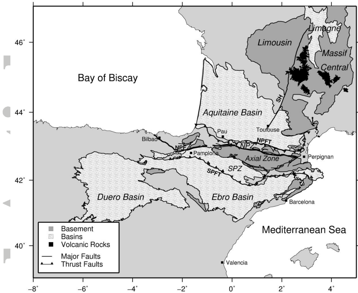
Figure 1. Main geological and structural units of the study region. NPF: North Pyrenean Fault, NPFT: North Pyrenean Front Thrust, SPFT: South Pyrenean Front Thrust, SH: Sillon Houiller (sometimes also referred to as the "Toulouse Fault"), NPZ: North Pyrenean Zone, SPZ: South Pyrenean Zone.
