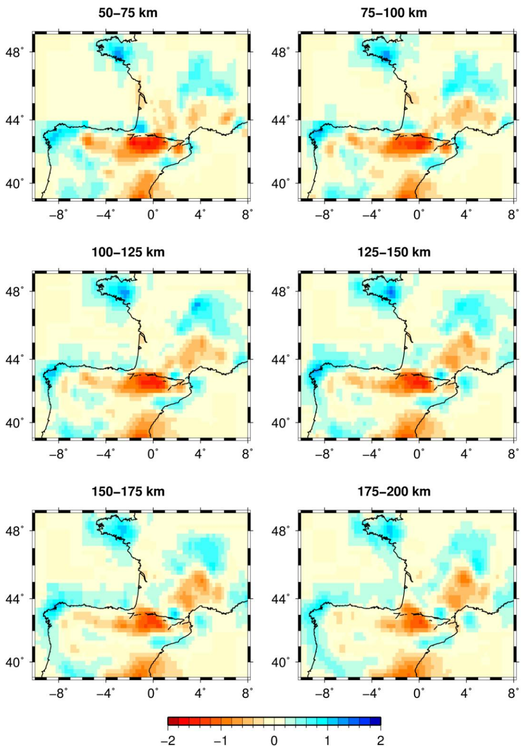
Figure 11. Map views of the P velocity model obtained after crustal corrections at 50, 75, 100, 125, 150, and 175 km depth. The color scale, in percents with respect to the ak135 reference Earth model, is the same in all the plots.
