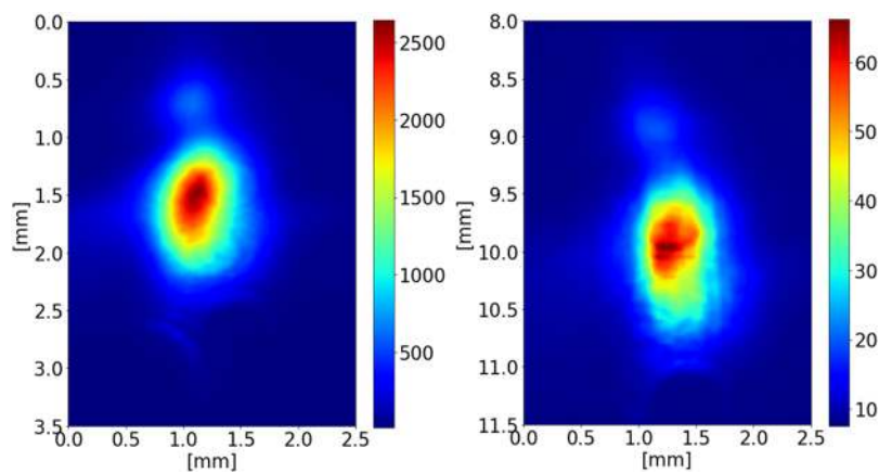
FIG. 2. A comparison of the beam profiles 80 m after the monochromators on a YAG-screen. On the left side is displayed the beam after two reflections from the highly polished Si (111) crystals. The right side shows the beam after the additional Si (533) monochromator without high quality polishing. Both images show the average over roughly 1800 shots of the FEL. This demonstrates that the spatial profile of the coherent FEL beam is preserved by the Si (533) channel-cut monochromator.
