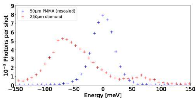
FIG. 7. Measured spectra from 50\ \mu\text{m} PMMA (blue) and 250\ \mu\text{m} single crystal diamond (red). The elastic signal from the PMMA shown here is reduced by a factor of 10. As it is a perfect single crystal, there is no quasielastic scattering from the diamond. Instead, there are the peaks corresponding to phonon creation and annihilation. The diamond spectrum is reproduced with permission from Descamps et al. , "An approach for the measurement of the bulk temperature of single crystal diamond using an x-ray free electron laser," Sci. Rep. 10 , 14564 (2020). Copyright 2020 Springer Nature Limited.
