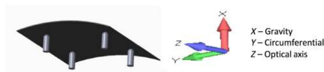
Fig. 5 Illustration of the four-point kinematic support of an x-ray mirror. The four supports are approximately located one quarter way inboard from each corner. See text for a discussion of the advantages of aligning and bonding a mirror segment using these four supports, which are also called spacers or posts.
