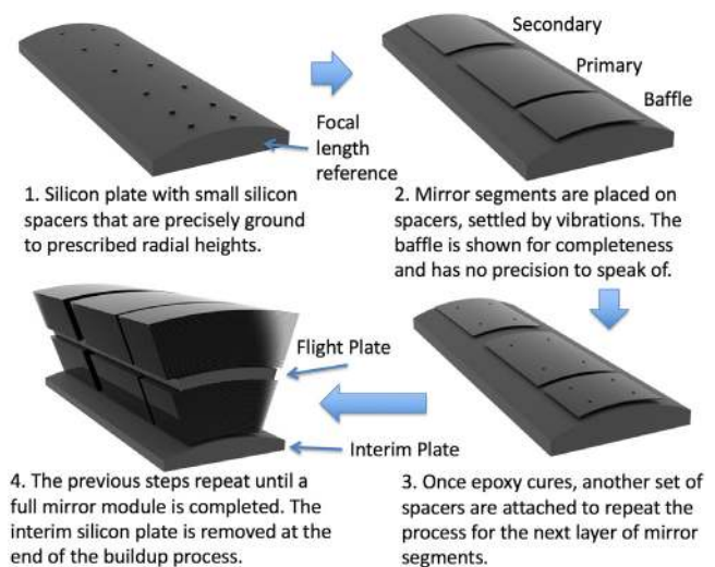
Fig. 8 Building-up of a mirror module. It is a repetition of fabrication, alignment, and bonding of one mirror segment after another. The interim plate is for the construction process only. It will be removed before the module is integrated into a metashell with the flight plate as its load-bearing structure and focal length reference.
