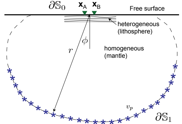
Figure A1. An effective configuration for lithospheric-scale SI. A medium with receivers (triangles) on the free surface is illuminated from below with a distribution of sources, of which the location is given in polar coordinates (r, \phi) .
