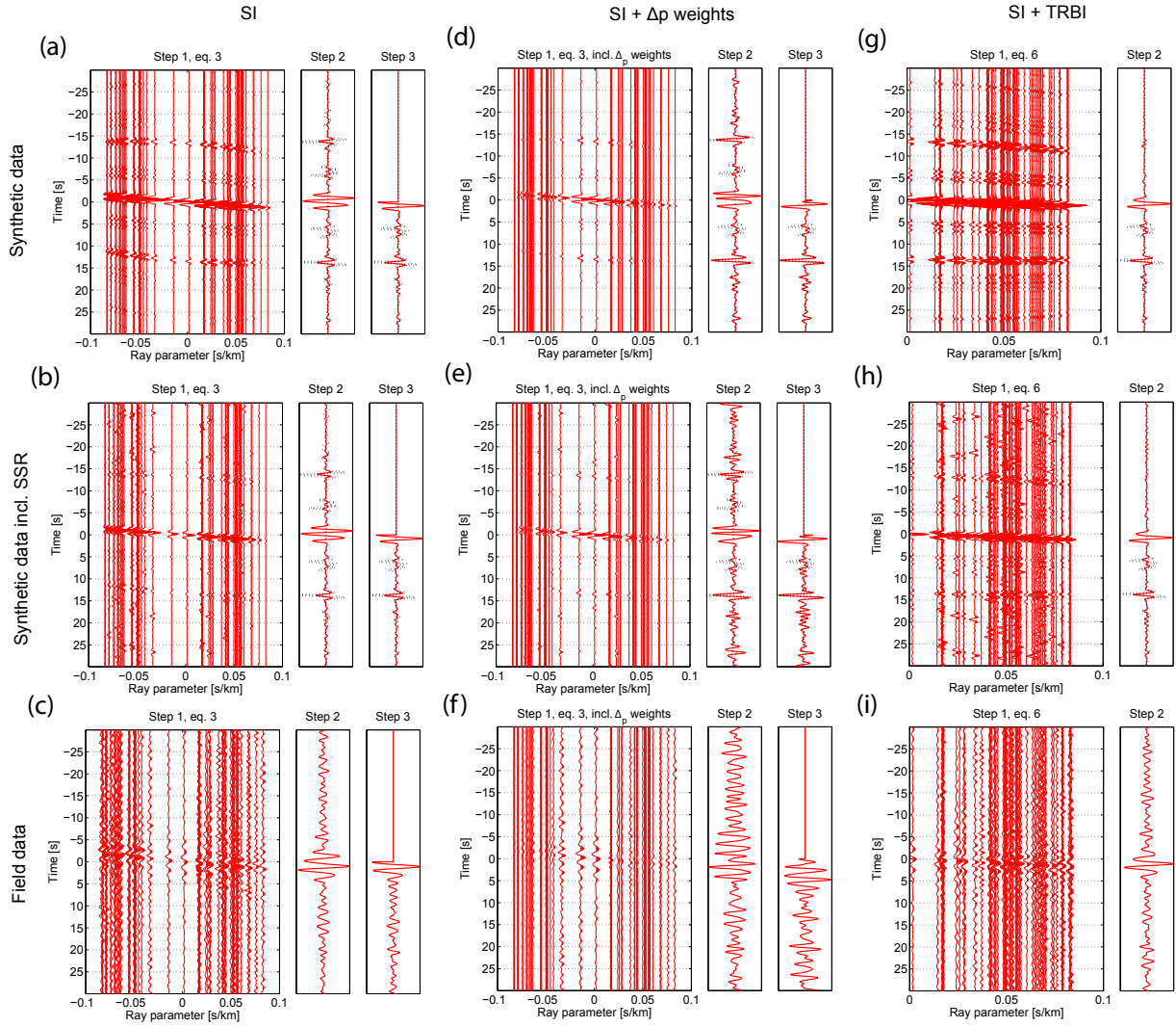
Figure A8. Visualization of the integrand (correlation panel) and integral (stack) of the seismic interferometric relations for \mathbf{x}_A and \mathbf{x}_B at station 16 and 8, respectively, for synthetic data (upper and middle panels) and the field data (lower panels). In the integrand displays, the traces are ordered as function of rayparameter. For the synthetic data, in step 2 and 3, a reference response is shown as a black dotted line. In (a)-(c) no adjustment is made for the irregular source distribution, in (d)-(f) every trace is weighted by its distance to the neighboring traces and for (g)-(i) the traces caused by effective sources with negative rayparameters are time-reversed and displayed at positive rayparameter. (a), (d) and (g) are for isolated P -phase responses, whereas (b), (e) and (h) are for direct wave responses 'polluted' with two source-side reverberations (e.g. pP and sP ) and (c), (f) and (i) are for the Laramie data from the field.
