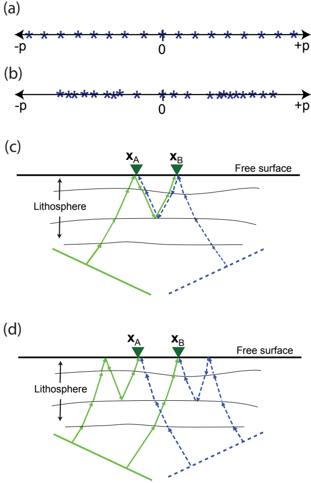
Figure 2. In (a) an ideal illumination is shown for plane-wave sources, expressed in rayparameters. In (b) a more realistic distribution of plane-wave sources is shown. In (c) and (d) examples of ray paths are indicated that in (c) do contribute to the retrieval of a reflection after crosscorrelation, but in (d) do not.
