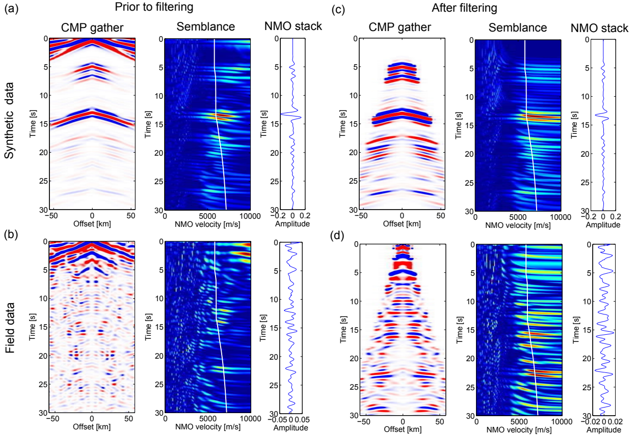
Figure 7. A common-midpoint gather, retrieved with seismic interferometry, for the midpoint position coinciding with station 12 (left), its semblance (middle) and normal-move-out stack (right), using the model velocity function v_p(t) as depicted by the white line in the semblance plot (middle). The same 3 panels are shown for the synthetic data (a), the field data (b) and the synthetic and field data after filtering, (c) and (d), respectively
