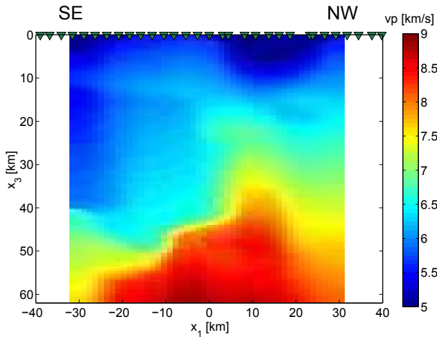
Figure 8. Estimated velocity model of the lithosphere below the Laramie array
