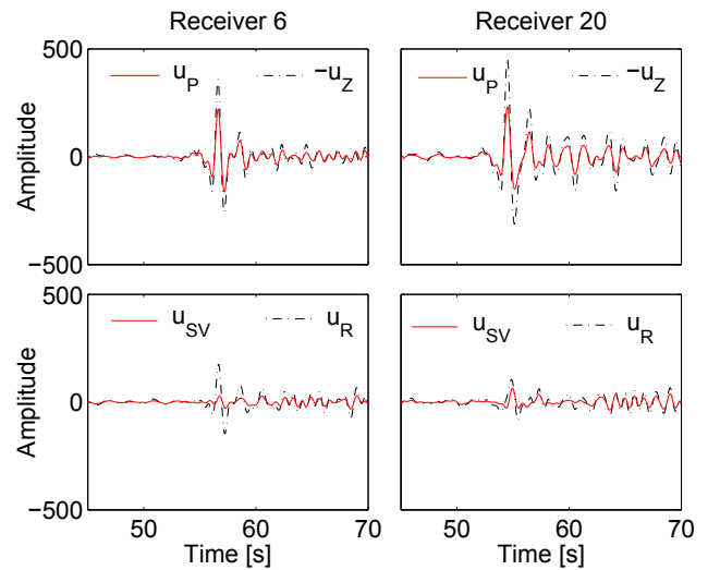
Figure A7. Particle velocity registration before ( u_Z, u_R ) and after ( u_P, u_{SV} ) decomposition for receiver 6 (left) and 20 (right). A time-window is shown which contains a P-phase arrival with p = 0.057 s/km.
