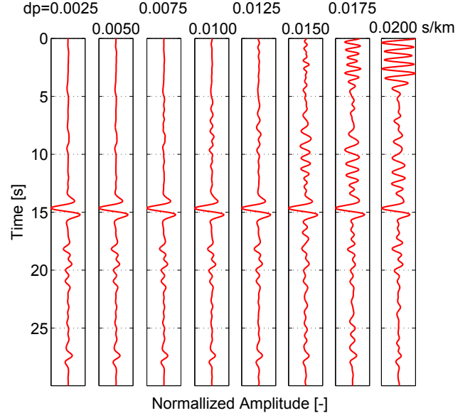
Figure A3. The result after applying SI to synthetic transmission responses, for obtaining a virtual source and a receiver at a distance of 40 km. From left to right, the rayparameter spacing of the transmission responses is increased from dp = 0.0025 to dp = 0.0200 s/km.
