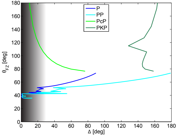
Figure A5. Extent of the Fresnel zone expressed in source-to-array azimuth ( \theta_{FZ} ) as a function of epicentral distance ( \Delta ) for four different P-wave phases. The gray shading depicts the distance range in which the approximations made for computing \theta_{FZ} are increasingly invalid.
