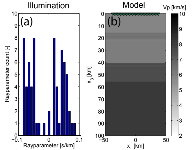
Figure 4. (a) A histogram distribution of the rayparameters of the selected phase responses. A bin size dp = 0.0083 s/km is taken, which corresponds to the required sampling of equation (4). (b) A simplified P-wave velocity model ( v_p ) for the crust and upper mantle, with 31 receivers (triangles) on the free surface.
