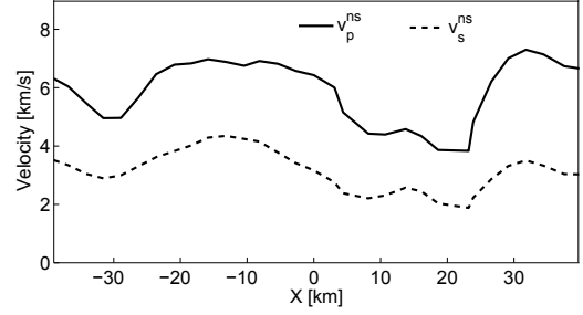
Figure A6. Estimated velocity model of the near surface.
