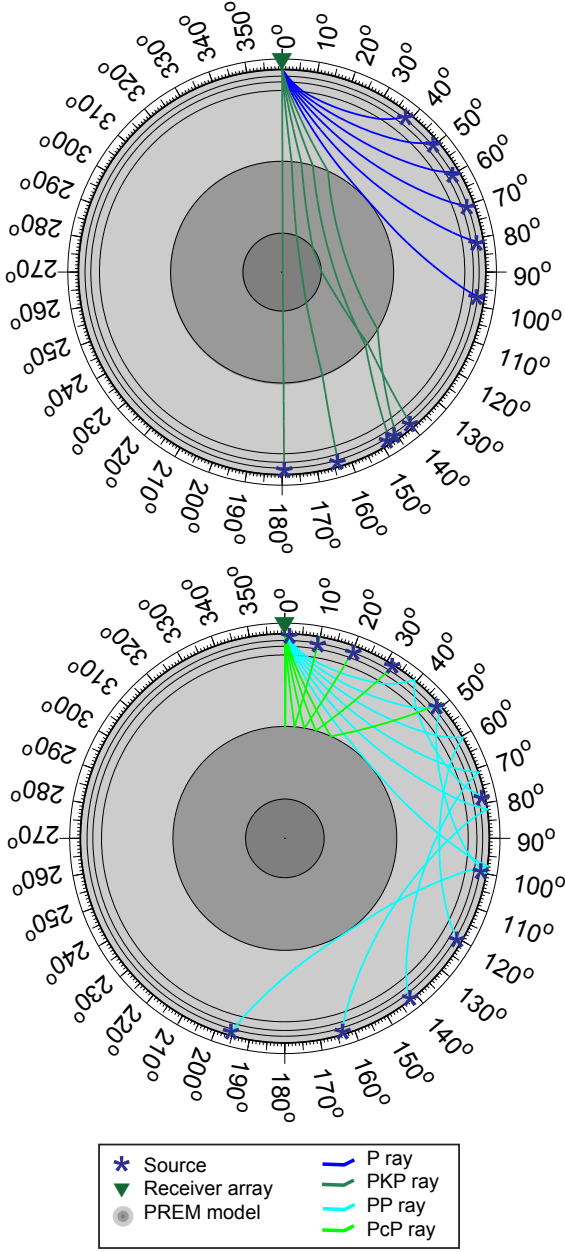
Figure A4. The source sampling required for lithospheric-scale SI, ray-traced to a distribution of earthquakes at regional, teleseismic and global distances. The minimum distribution for P and PKP phases (up) and for PP and PcP phases (down).
