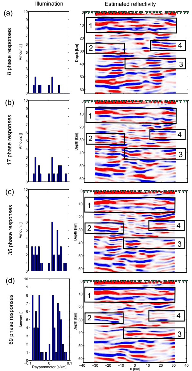
Figure A9. (left) The rayparameter distribution of a subset of phase responses and (right) the resulting image using only this subset of phase responses. The images are obtained using (a) 8, (b) 17, (c) 35 and (d) 69 phase responses.
