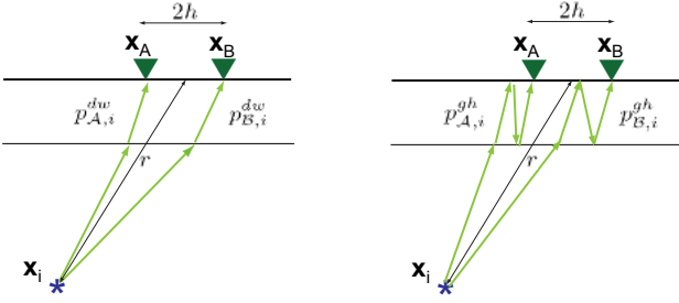
Figure A2. The raypaths for two direct waves (left) and two ghost reflections (right)
