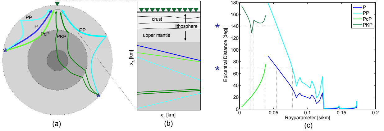
Figure 1. (a) A depiction of the raypaths for different P-wave phases between two earthquake sources (stars) and a regional array of receivers (triangle). For the teleseismic source (left) P , PP and PcP are shown while for the global source (right) PKP and its branch through the inner core ( PKIKP ) are shown. (b) An enlargement of the subsurface below the array with the wavefronts of the different phases (colored dipping lines) traveling upwards, just before they hit the lithosphere from below. The lateral ( x_1 ) and depth axis ( x_3 ) have equal scaling. The wavefronts are depicted with only half the dip of what may be expected. In reality, the different phases arrive near the array with a considerable time lapse. (c) The different phases as a function of epicentral distance ( \Delta ) and absolute rayparameter |p| for which they exist (Knapmeyer 2004). From this graph can be read, the |p| of the phases caused by the teleseismic source ( \Delta = 70^\circ ) and the global source ( \Delta = 140^\circ ).
