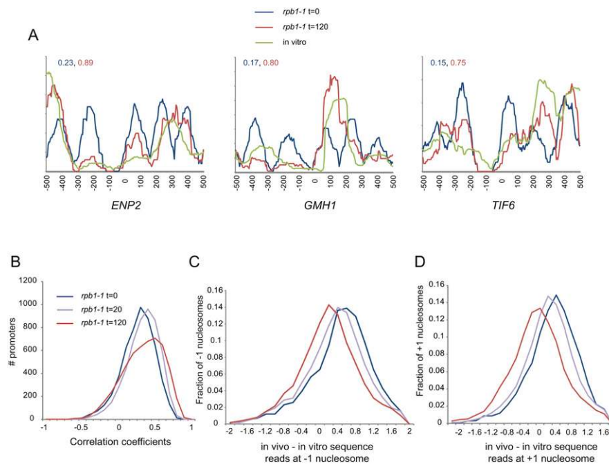
Figure 5. Nucleosomes relax toward in vitro preferred locations after Pol II loss. (A) Three examples of promoters where data from Pol II inactivation matches in vitro nucleosome assembly data better than data from before Pol II inactivation. Shown are extended read coverage along 1000 bp centered on TSS. Numbers shown in the inset are correlations between in vitro coverage and t=0 (blue) and t=120 (red) in vivo coverage. (B) Promoter chromatin architecture globally shifts toward in vitro preferences as polymerase is inactivated. Extended read coverage along the 1 kb centered on the TSS was extracted for all genes, and correlation coefficients were calculated to equivalent data for in vitro nucleosome reconstitution experiments (Kaplan et al. 2008). Histograms show a global shift of promoters toward the in vitro nucleosome pattern. (C) Normalized occupancy of -1 nucleosomes better matches in vitro data after polymerase loss. For all -1 nucleosomes (called at t=0 or at t=120 ), the difference between in vivo normalized occupancy and in vitro normalized occupancy at the center of the in vivo nucleosome were calculated and presented as a histogram. (D) As in C, but for all +1 nucleosomes.
