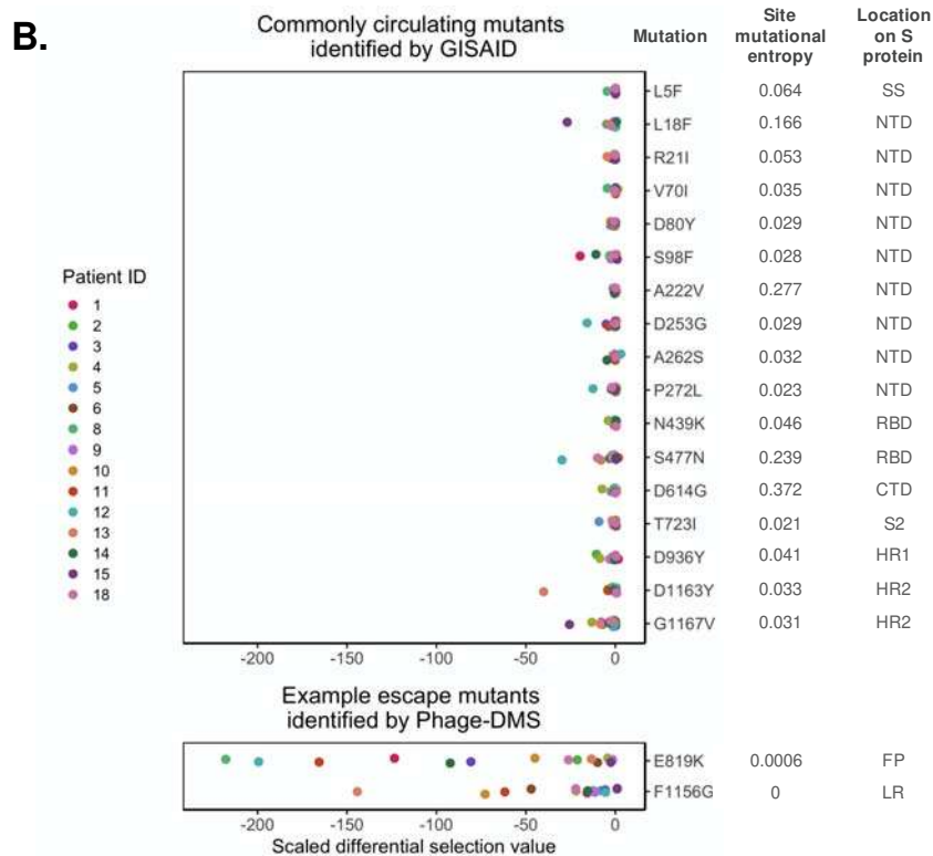
Figure 5. Predicted effects of commonly circulating S protein variants on antibody escape. (A) Scatterplot comparing the effect of mutations on patient plasma antibody binding and the frequency of all circulating S protein variants. The mutational entropy of every circulating protein variant, as reported at the https://cov.lanl.gov website and based on GISAID global sequencing, is plotted on the x-axis. The average of the scaled differential selection values for all mutants at each site is plotted on
