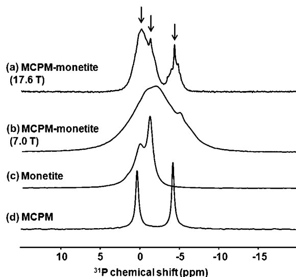
FIG. 5. ^{31}\text{P} MAS NMR spectra (a) ^{17}\text{O} -labeled MCPM-monetite at 17.6 T (3.2 mm, recycle delay: 90 s, number of scans: 16, \nu_{\text{rot}} : 24 kHz, ^1\text{H} decoupling). (b) ^{17}\text{O} -labeled MCPM-monetite at 7.0 T (4 mm, recycle delay: 30 s, number of scans: 16, \nu_{\text{rot}} : 14 kHz, ^1\text{H} decoupling). (c) Unlabeled monetite at 7.0 T (4 mm, recycle delay: 30 s, number of scans: 16, \nu_{\text{rot}} : 14 kHz, ^1\text{H} decoupling). (d) Unlabeled MCPM at 7.0 T (4 mm, recycle delay: 30 s, number of scans: 4, \nu_{\text{rot}} : 14 kHz, ^1\text{H} decoupling). Vertical arrows: \text{P}^{16}\text{O}_4 resonances.
