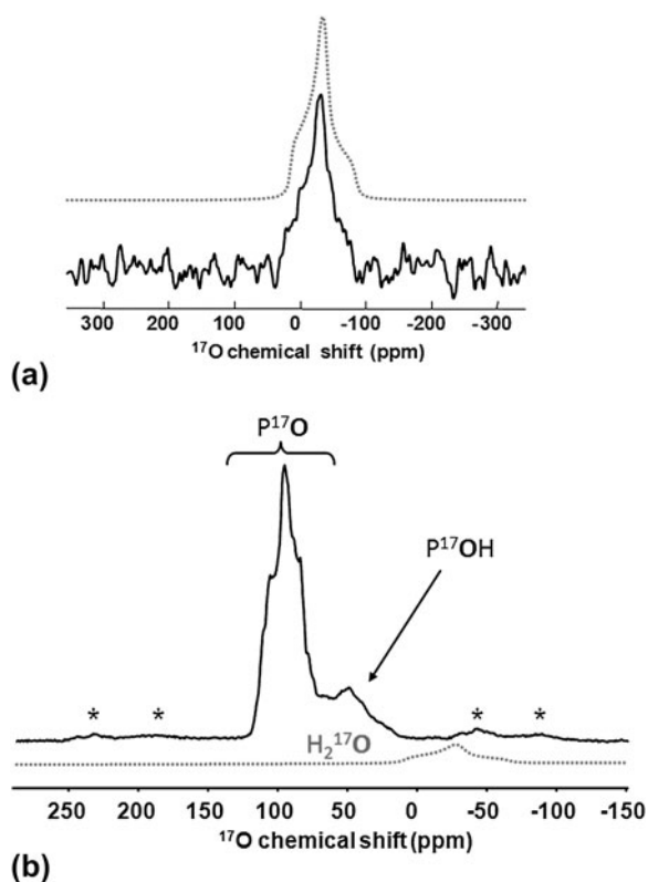
FIG. 1. (a) ^{17}\text{O} MAS NMR spectrum of MCPM at 14.1 T (3.2 mm rotor, recycle delay: 5 s, number of scans: 17196, \nu_{\text{rot}} : 20 kHz, ^1\text{H} decoupling). The dotted spectrum corresponds to a simulation 61 with a second-order quadrupolar interaction. (b) ^{17}\text{O} Hahn echo MAS NMR spectrum of MCPM-monetite at 17.6 T (4 mm, recycle delay: 15 s, number of scans: 64, \nu_{\text{rot}} : 14 kHz, ^1\text{H} decoupling). The dotted spectrum corresponds to the expected \text{H}_2^{17}\text{O} signal of MCPM with the quadrupolar parameters given in the text (and the intensity expected with respect to the composition of the sample). * ^* spinning side bands; MAS, Magic Angle Spinning; NMR, Nuclear Magnetic Resonance; MCPM, monocalcium phosphate monohydrate.
