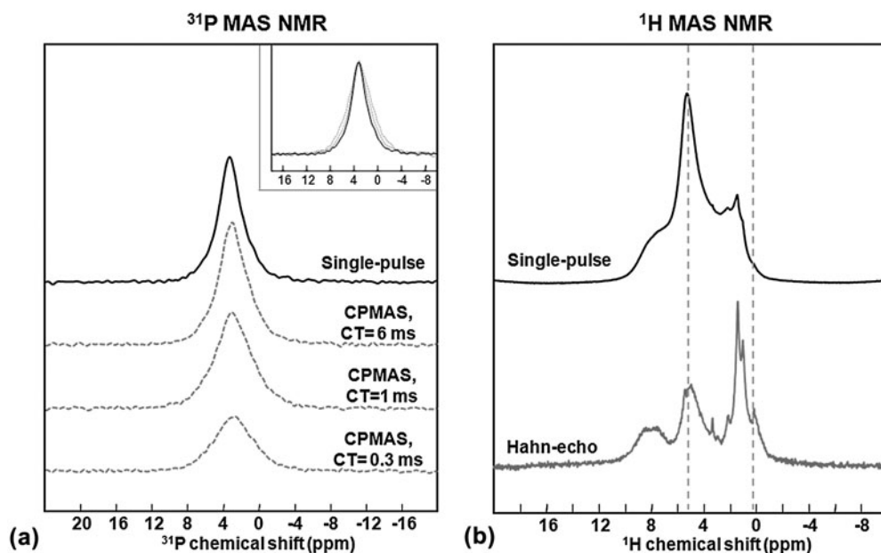
FIG. 10. (a) ^{31}\text{P} single-pulse spectrum (in black, top) and ^1\text{H}/^{31}\text{P} CPMAS spectra (in grey, bottom), recorded with contact times of 0.3, 1.0, and 6.0 ms. The inset at the top right compares the line widths of the single-pulse spectrum with those of the CPMAS spectra recorded with contact times of 1 and 6 ms (the breadth of the phosphate peak varies as indicated in the text). (b) ^1\text{H} NMR spectra recorded using the single-pulse sequence (in black, top) and the Hahn echo sequence (in grey, bottom). Details on all the acquisition parameters can be found in the experimental section of the manuscript.
