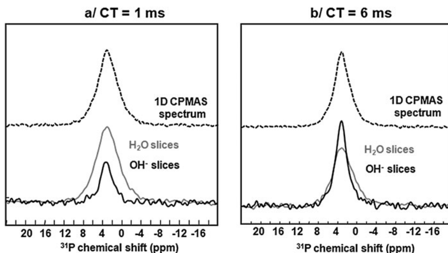
FIG. 12. Top spectra: 1D ^1\text{H} \rightarrow ^{31}\text{P} CPMAS spectra (recorded with contact times of 1.0 and 6.0 ms). Bottom spectra: ^{31}\text{P} NMR cross sections of the 2D ^1\text{H} - ^{31}\text{P} HETCOR spectra, corresponding to the \text{OH}^- (in black) and \text{H}_2\text{O} (in grey) signals.
