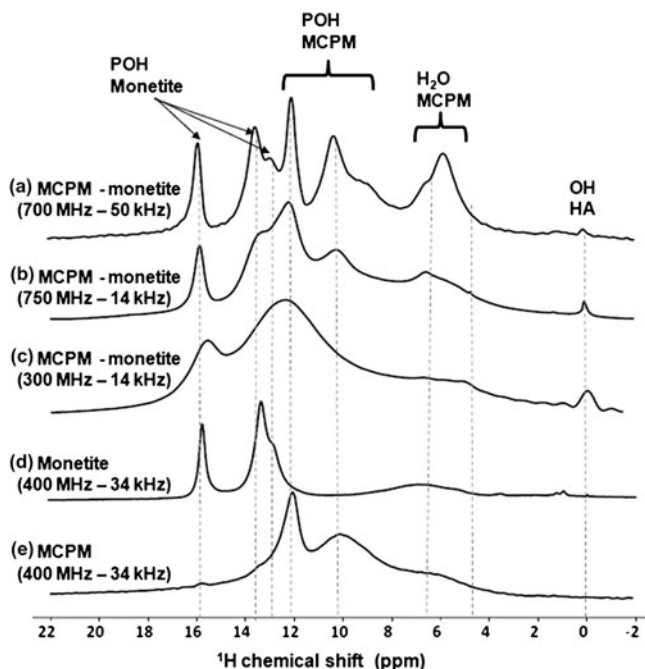
FIG. 7. ^1\text{H} NMR spectra of MCPM-monetite at various fields and the nonlabeled corresponding pure phases, and various spinning speeds \nu_{\text{rot}} [4 mm (14 kHz), 2.5 mm (34 kHz), 1.3 mm (50 kHz), recycle delay: from 5 to 60 s, number of scans: 8]. (d) The spectrum of monetite shows the presence of water signals at \sim 4 to 7 ppm, suggesting that this phase was not well dried before the NMR measurement.
