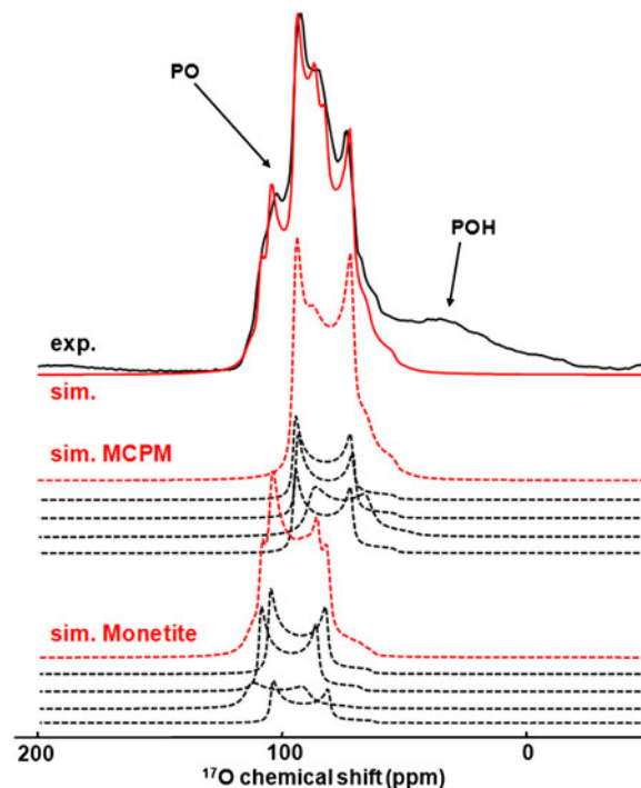
FIG. 4. ^{17}\text{O} MAS NMR spectrum of MCPM-monetite at 14.1 T in black, top spectrum. The simulation in the PO region (in red, top) corresponds to the sum of the contributions of MCPM and monetite (the isotropic chemical shifts were extracted from the DOR data, the quadrupolar parameters were estimated from GIPAW calculations—see text for further details).
