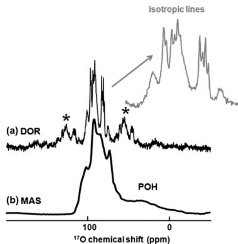
FIG. 3. (a) ^{17}\text{O} DOR NMR spectrum of MCPM-monetite at 14.1 T (recycle delay: 1 s, number of scans: 5000, inner \nu_{\text{rot}} : 6.50 kHz, outer \nu_{\text{rot}} : 1.44 kHz, no ^1\text{H} decoupling). Only the \text{P}^{17}\text{O} groups are detected. ‘*’ spinning side bands. In red: expansion of the DOR spectrum showing the J doublets ( ^1\text{J}_{\text{O-P}} couplings). The \text{P}^{17}\text{OH} resonances are not detected (no ^1\text{H} decoupling, see text). (b) The corresponding ^{17}\text{O} echo MAS NMR spectrum at 14.1 T (4 mm, recycle delay: 20 s, number of scans: 3200, \nu_{\text{rot}} : 12.5 kHz, ^1\text{H} decoupling). In this case the \text{P}^{17}\text{OH} signals are observed. DOR, double rotation.
