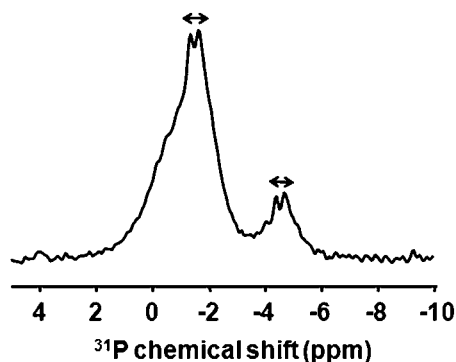
FIG. 6. \{^{31}\text{P}\text{-}^{17}\text{O}\} J-MAS-HM-QC NMR spectrum of MCPM-monetite at 17.6 T (3.2 mm, recycle delay: 120 s, number of scans: 64, \nu_{\text{rot}} : 24 kHz, \tau = 3.6 ms, ^1\text{H} decoupling).
