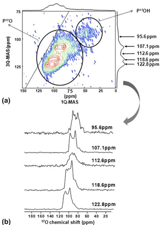
FIG. 2. (a) ^{17}\text{O} 3Q-MAS NMR spectrum of MCPM–monetite at 17.6 T (3.2 mm, recycle delay: 2 s, \nu_{\text{rot}} : 24 kHz, ^1\text{H} decoupling). The \text{P}^{17}\text{O} and \text{P}^{17}\text{OH} regions are indicated. (b) Isotropic contributions to the highly resolved dimension and the corresponding MAS lineshapes.
