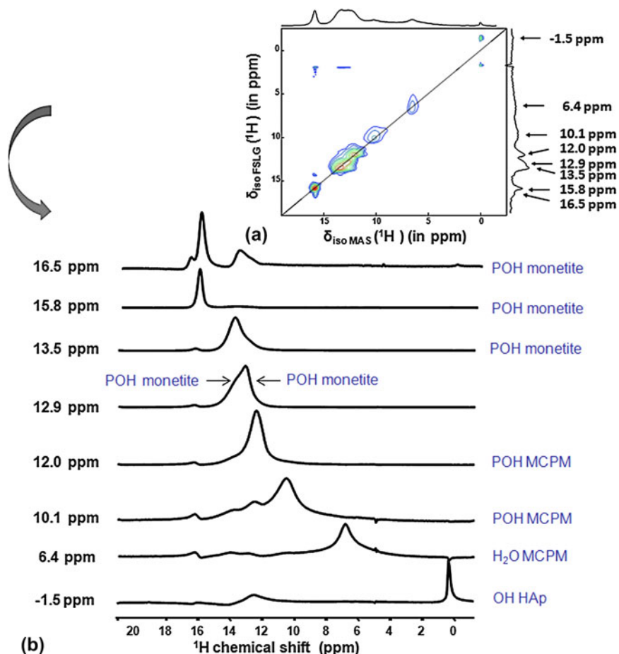
FIG. 8. (a) ^1\text{H} - ^1\text{H} 2D Frequency Switched Lee Goldberg NMR spectrum of MCPM-monetite at 17.6 T (4 mm, recycle delay: 5 s, number of scans: 16, \nu_{\text{rot}} : 14 kHz). (b) The corresponding isotropic contributions.
