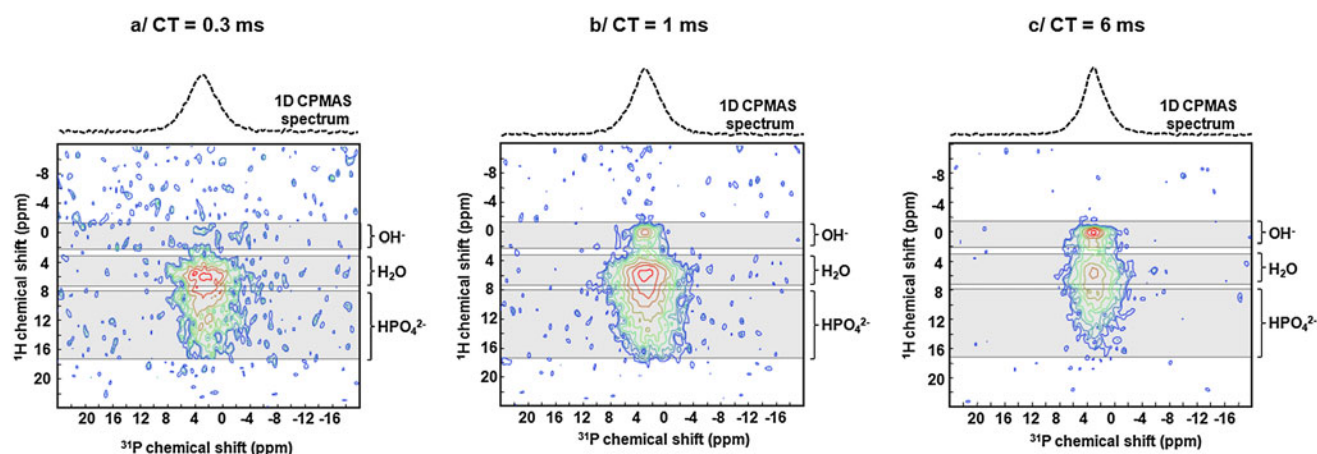
FIG. 11. 2D ^1\text{H} - ^{31}\text{P} HETCOR CPMAS NMR spectra recorded using contact times of a/0.3, b/1.0, and c/6.0 ms, respectively. HETCOR, heteronuclear-correlation.
