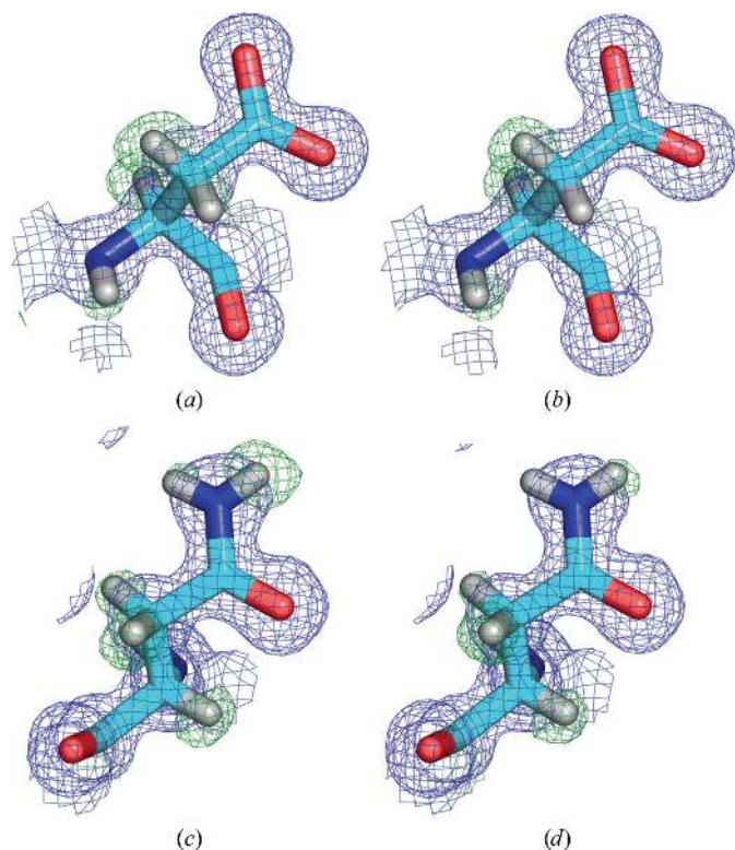
Figure 5 Comparison of the models of recombinant thaumatin I and plant thaumatin I around Asn104 and Asp113. The OMIT maps of recombinant thaumatin I are shown in (a) for Asp113 ( B factors: OD1, 7.74 Å 2 ; OD2, 9.28 Å 2 ) and (c) for Asn104 ( B factors: ND2, 6.78 Å 2 ; OD1, 7.21 Å 2 ). In contrast, the OMIT maps of plant thaumatin I are shown in (b) for Asp113 ( B factors: OD1, 8.59 Å 2 ; OD2, 10.19 Å 2 ) and (d) for Asn104 ( B factors: ND2, 7.40 Å 2 ; OD1, 7.93 Å 2 ). The \sigma_A -weighted 2mF_o - DF_c maps contoured at 1.0\sigma are drawn in blue and the mF_o - DF_c maps omitting H atoms contoured at 3.0\sigma are shown in green.
