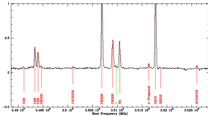
Fig. 11. Two 2.5 GHz XFFTS boards combined, with 500 MHz overlap, to create a 4 GHz-wide spectrometer. The sample spectrum, part of a Galactic Center line survey (Güsten, priv comm.), shows the upper sideband of the sideband separating APEX/FLASH + receiver.
