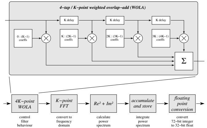
Fig. 6. Block diagram of the polyphase filter bank (PFB) signal processing pipeline. The PFB not only produces a flat response across the passband, but also excellently suppresses of out-of-band signals.
