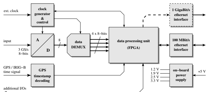
Fig. 3. Block diagram of the 1.5 GHz bandwidth AFFTS digitizer/analyzer board. The board can be equipped with a single- or dual-input ADC (National ADC083000 or ADC08D1500). The optional GigaBit-ethernet interface allows high-speed data acquisition with transfer rates of up to 90 MBytes/s, which are required for pulsar/transient search or to readout MKIDs – Microwave Kinetic Inductance Detectors.
